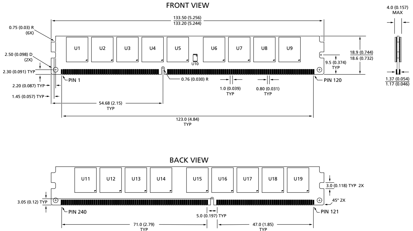
Figure 3: 240-Pin DDR3 UDIMM
