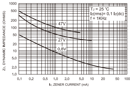
FIG.3- EFFECT OF ZENER CURRENT ON ZENER IMPEDANCE
