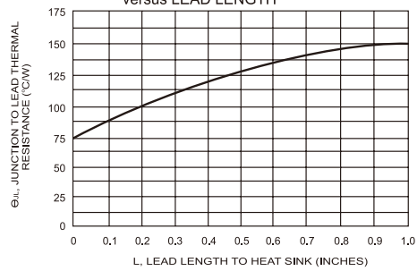
FIG.9- TYPICAL THERMAL RESISTANCE versus LEAD LENGTH
