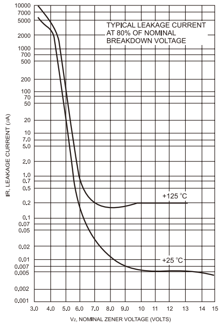
FIG.5- TYPICAL LEAKAGE CURRENT
