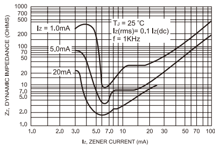
FIG.4- EFFECT OF ZENER VOLTAGE ON ZENER IMPEDANCE
