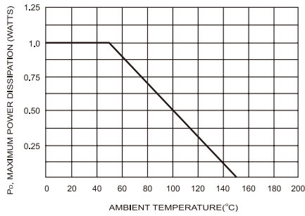
FIG.1- POWER TEMPERATURE DERATING CURVE
