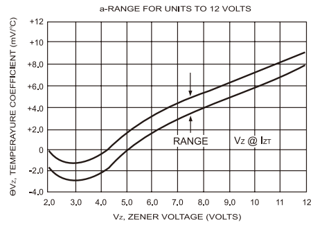
FIG.7- TEMPERATURE COEFFICIENTS
