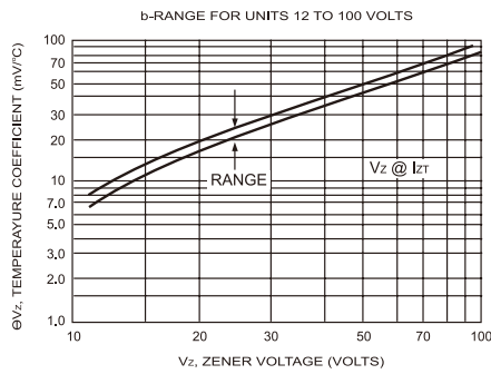
FIG.7- TEMPERATURE COEFFICIENTS
