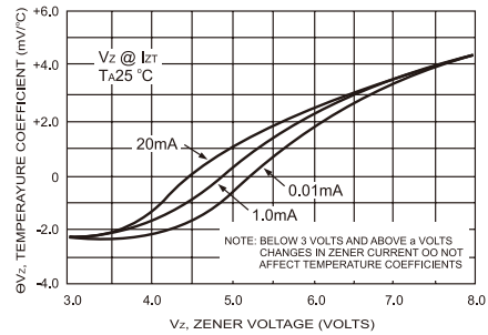
FIG.8- EFFECT OF ZENER CURRENT
