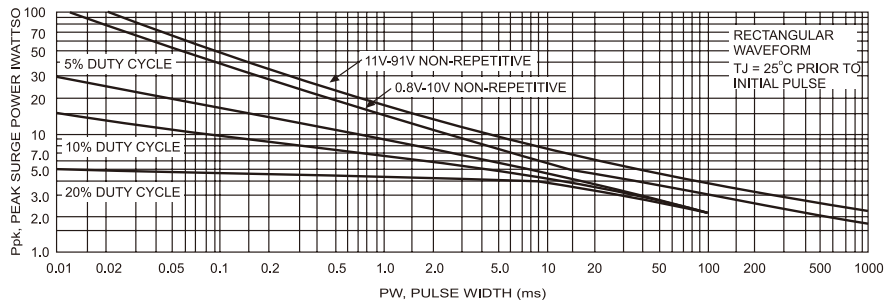
FIG.10- MAXIMUM SURGE POWER
