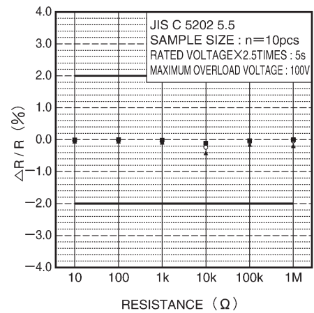
Fig.7 Short time overload
