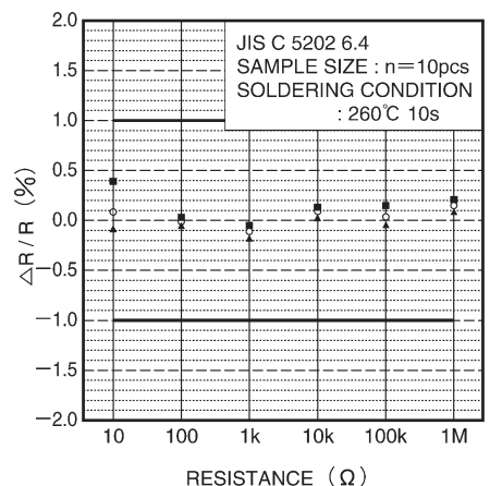
Fig.10 Resistance to soldering heat
