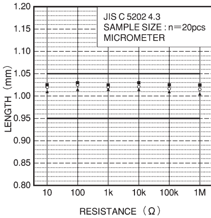
Fig.2 Dimensions (length)
