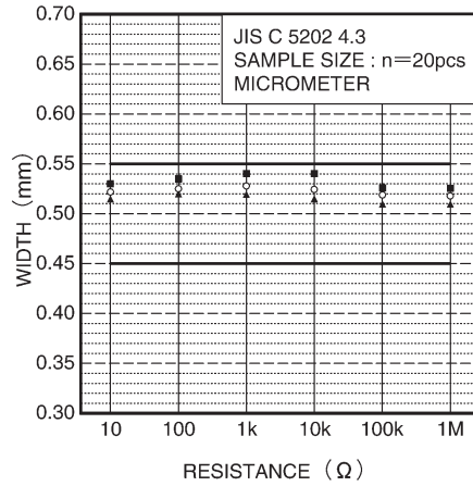
Fig.3 Dimensions (width)
