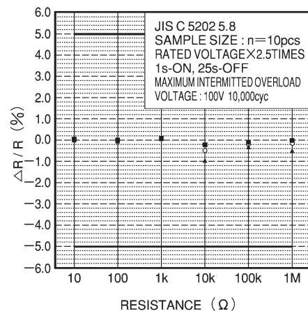
Fig.8 Intermittent overload
