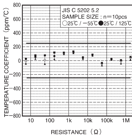
Fig.6 Resistance temperature characteristics
