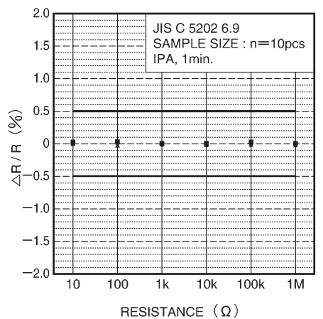
Fig.16 Resistance to solvents
