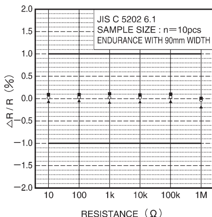
Fig.9 terminal strength (bending strength characteristics)
