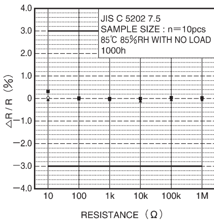
Fig.14 Humidity resistance (steady state)
