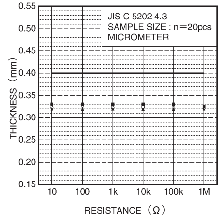
Fig.4 Dimensions (thickness)
