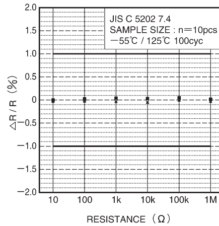
Fig.15 Temperature cycling
