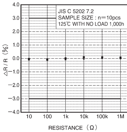
Fig.11 Resistance to dry heat
