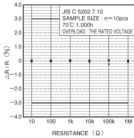
Fig.12 Endurance (rated load)
