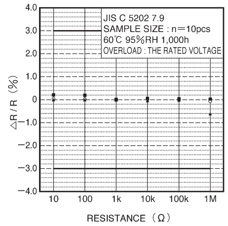
Fig.13 Endurance (under load in damp environment)
