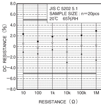
Fig.5 DC resistance
