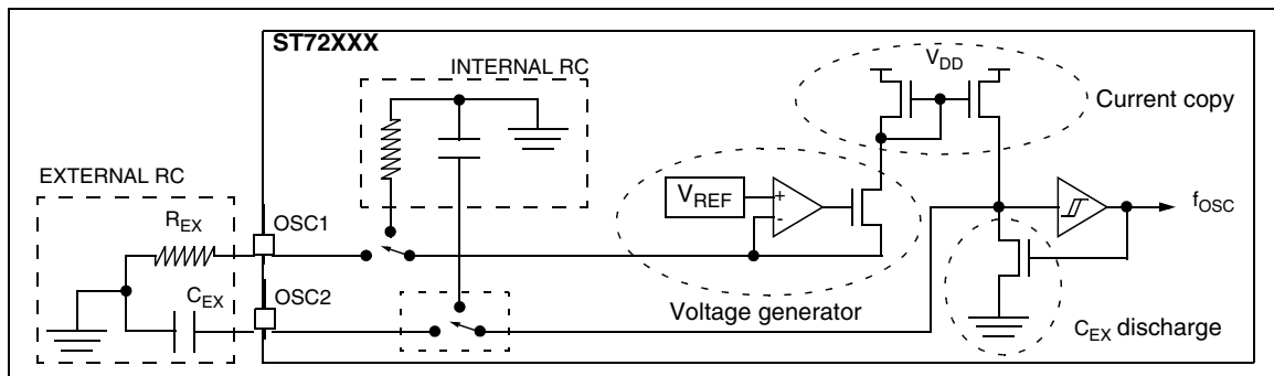
Figure 70. Typical Internal RC Oscillator
