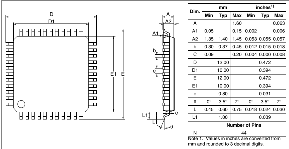
Figure 100. 44-Pin Thin Quad Flat Package (10x10)
