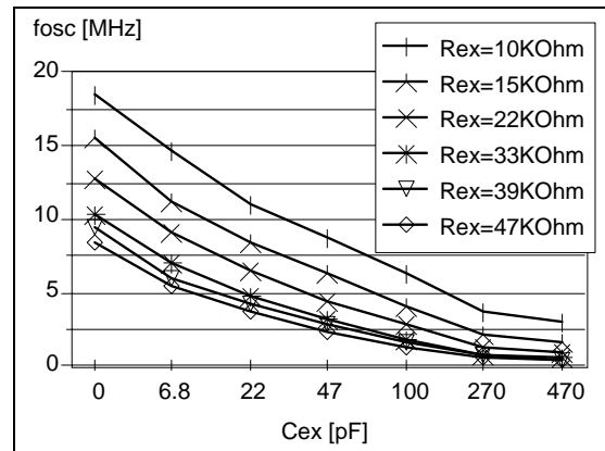
Figure 71. Typical External RC Oscillator
