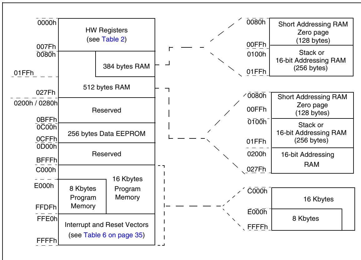
Figure 4. Memory Map
