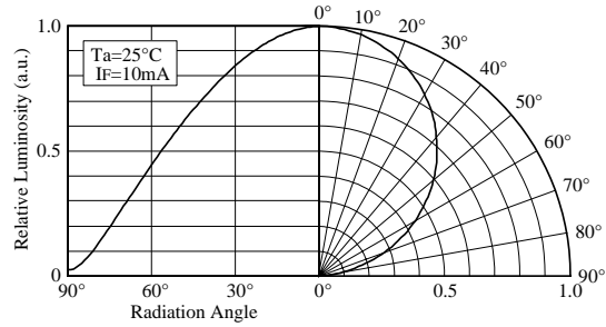
■ Directivity (NECW425B)
