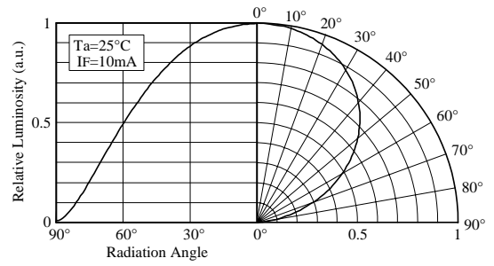
■ Directivity (NECB426B)
