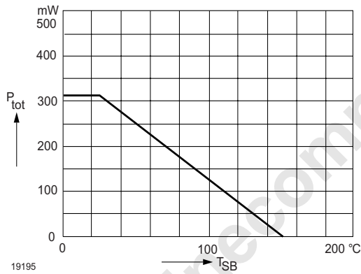
Figure 1. Admissible Power Dissipation vs. Temperature of Substrate Backside
