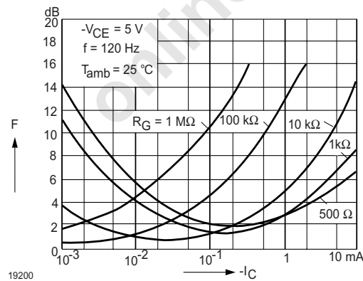
Figure 11. Noise Figure vs. Collector Current
