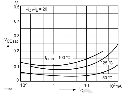
Figure 6. Collector Saturation Voltage vs. Collector Current
