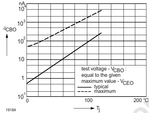
Figure 4. Collector-Base Cutoff Current vs. Ambient Temperature
