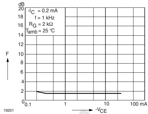
Figure 12. Noise Figure vs. Collector Emitter Voltage
