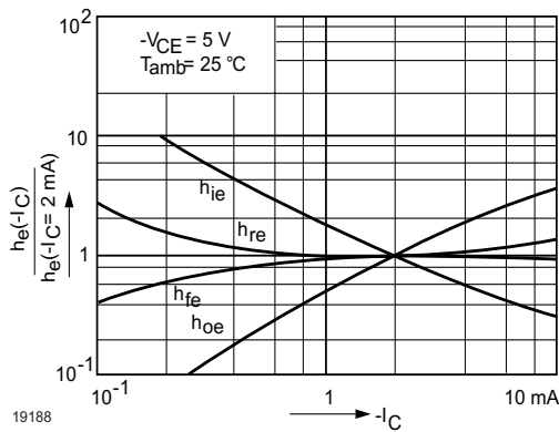
Figure 8. Relative h-Parameters vs. Collector Current
