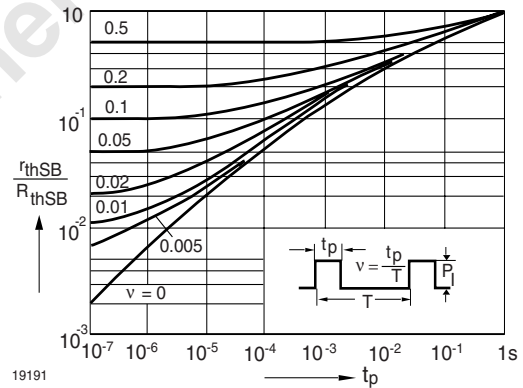
Figure 2. Pulse Thermal Resistance vs. Pulse Duration (normalized)
