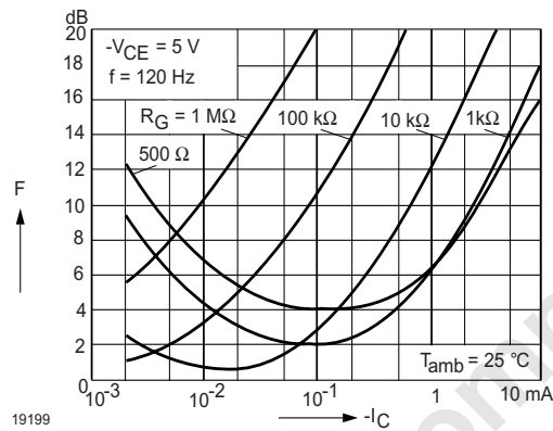
Figure 10. Noise Figure vs. Collector Current
