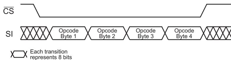
Figure 5-1. Chip Erase
