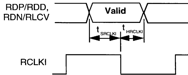
Fig. 27 Digital Receive Interface Input Timing Diagram
