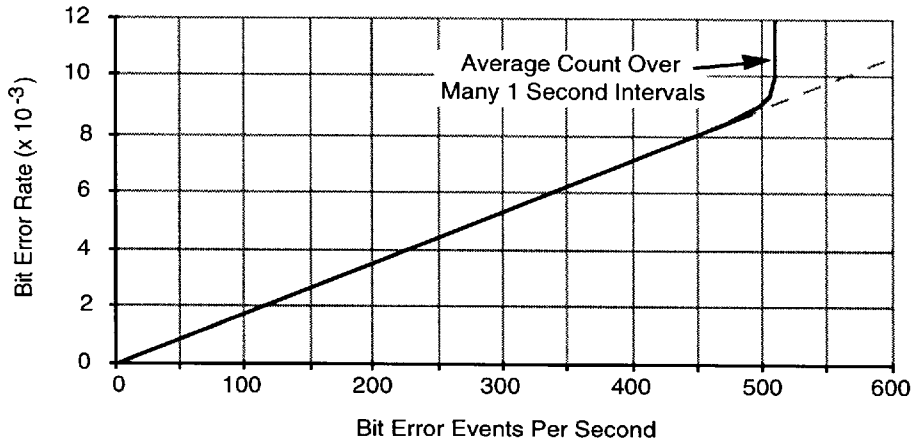
Fig. 21 BEE Count vs. BER for T1DM Framing Format
