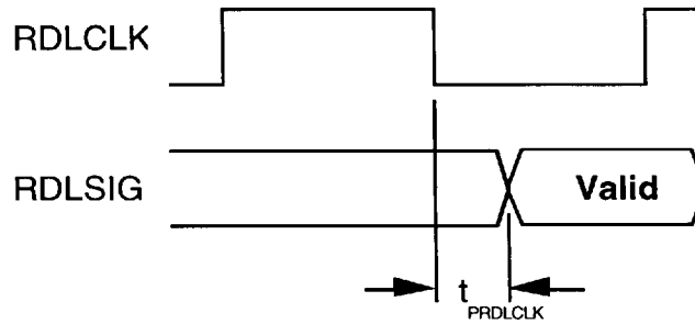
Fig. 30 Receive Data Link Output Timing Diagram
