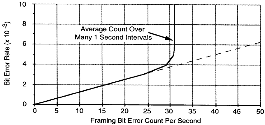
Fig. 16 FER Count vs. BER for SLC@96 Framing Format
