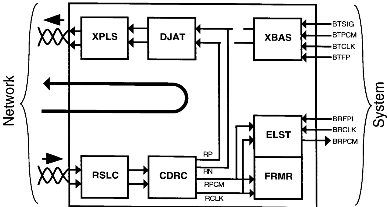
Fig. 9 Line Loopback
