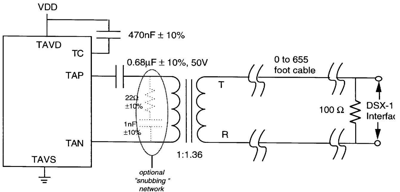
Fig. 6 External Analog Transmit Interface Circuit
