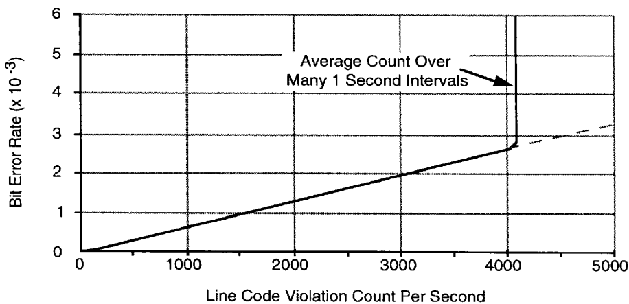
Fig. 14 LCV Count vs. BER
