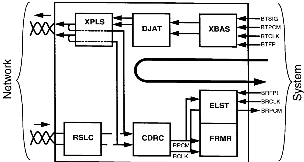
Fig. 11 Diagnostic Metallic Loopback
