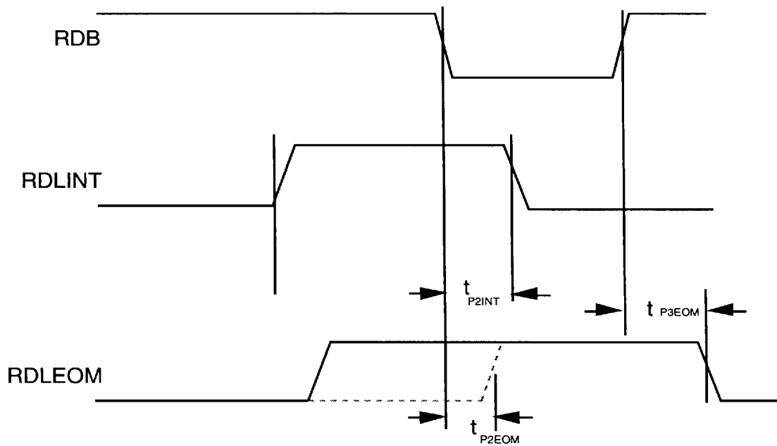
Fig. 35 Receive Data Link DMA Interface Output Timing Diagram
