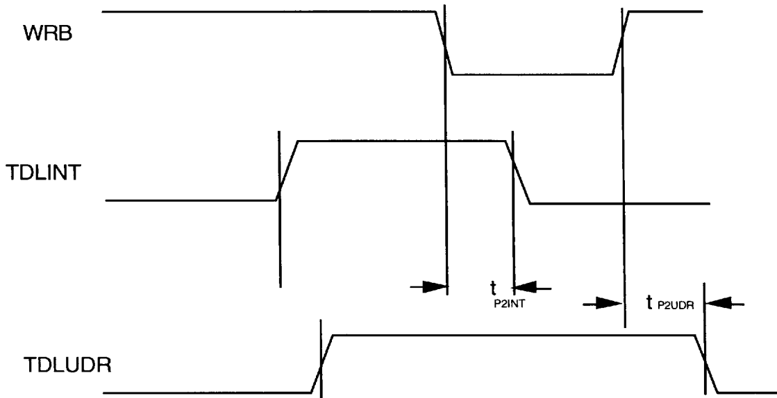
Fig. 34 Transmit Data Link DMA Interface Output Timing Diagram
