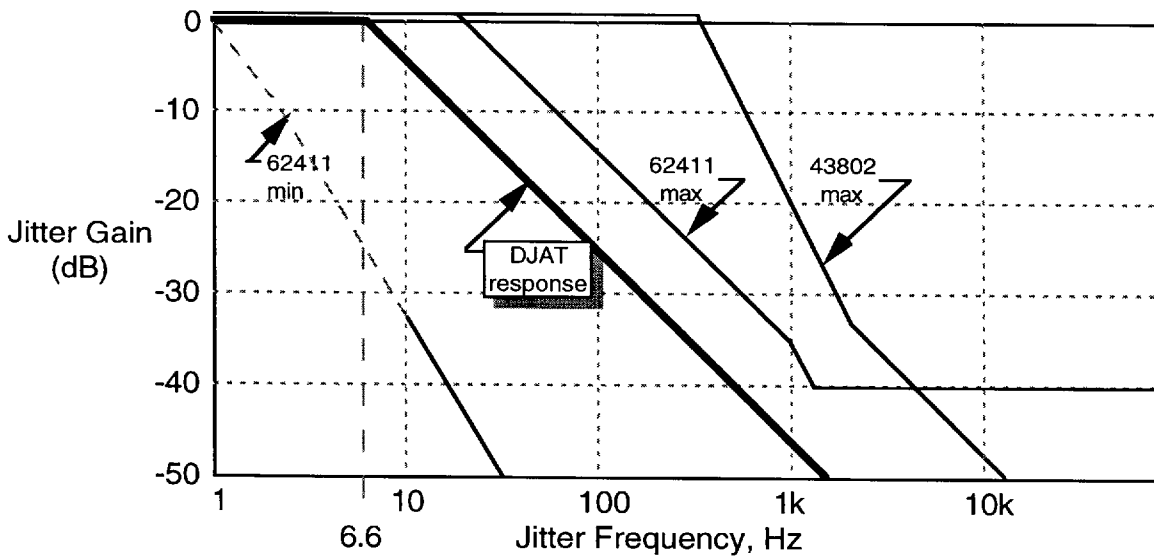
Fig. 5 DJAT Jitter Transfer
