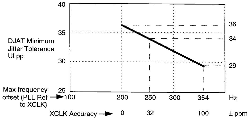
Fig. 4 DJAT Minimum Jitter Tolerance vs XCLK Accuracy
