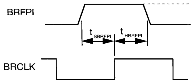
Fig. 29 Backplane Receive Input Timing Diagram
