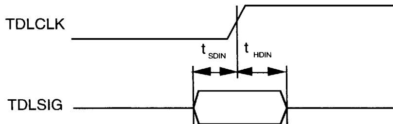
Fig. 28 Transmit Data Link Input Timing Diagram
