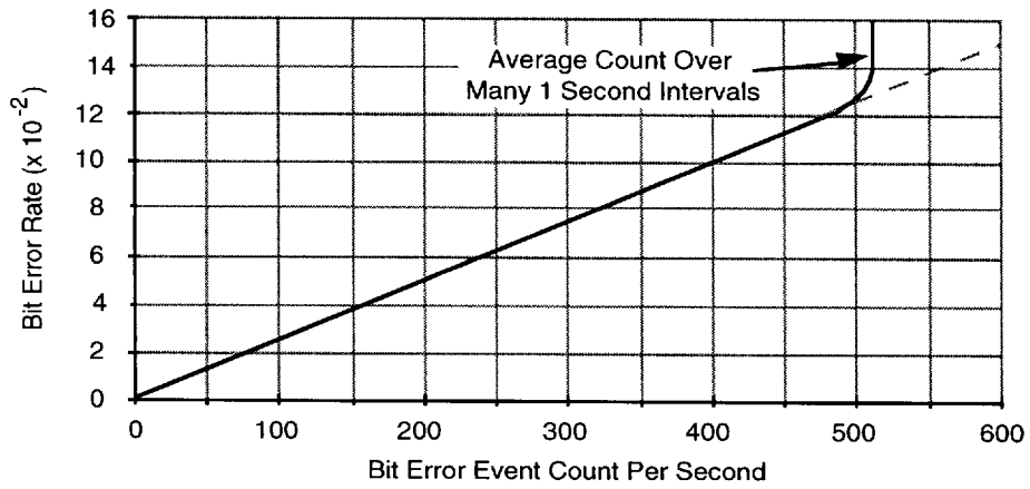
Fig. 20 BEE Count vs. BER for SLC@96 Framing Format
