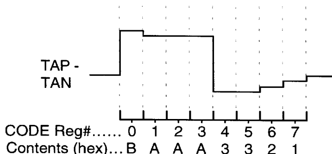
Fig. 13 CODE Register Sequence For 0-110 feet Build-out
