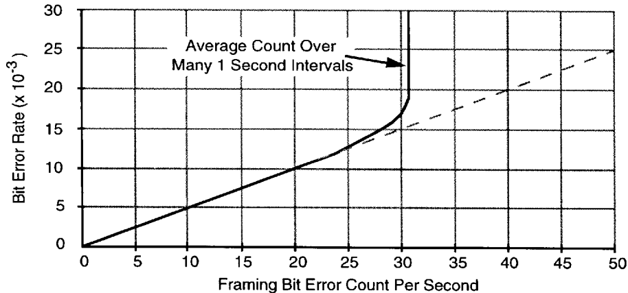
Fig. 18 BEE Count vs. BER for ESF Framing Format
