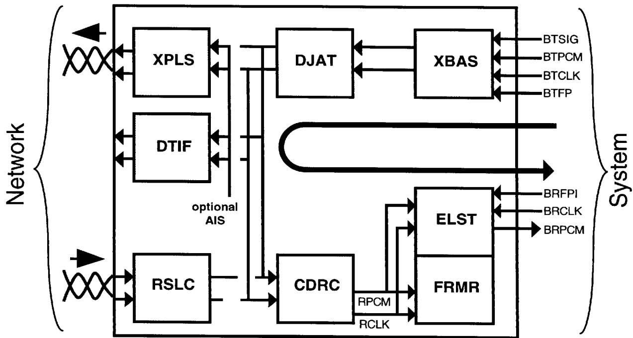
Fig. 10 Diagnostic Digital Loopback
