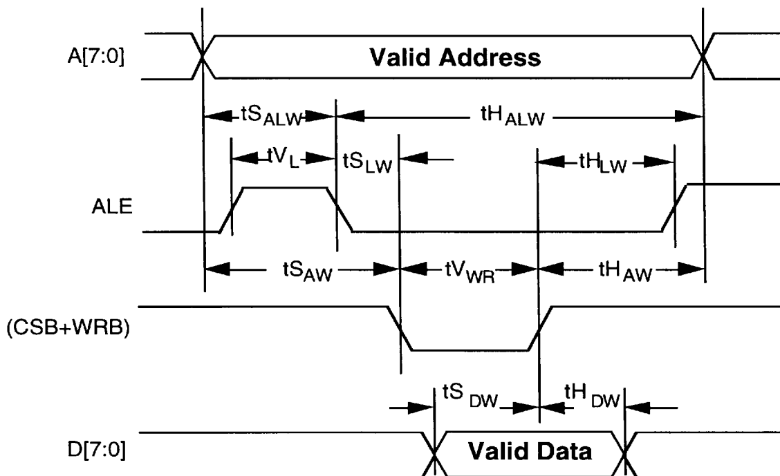
Fig 23 Microprocessor Write Access Timing
