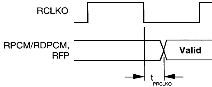
Transmit Interface Output Timing (Fig. 33)
