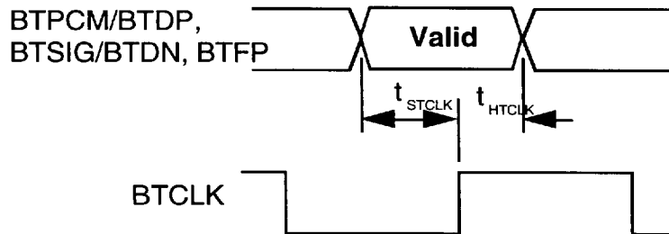
Fig. 24 Backplane Transmit Input Timing Diagram
