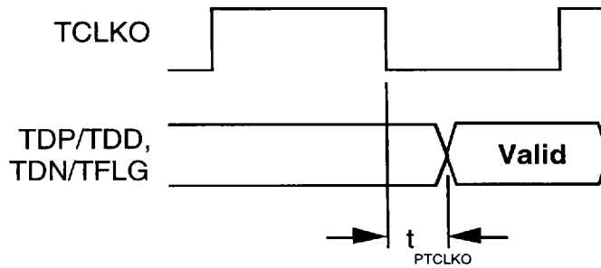
Fig. 33 Transmit Interface Output Timing Diagram
