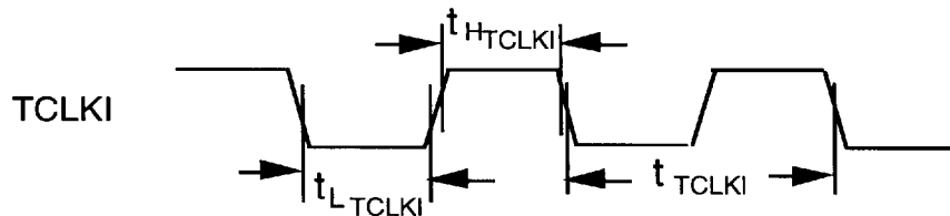
Fig. 26 TCLKI Input Timing
