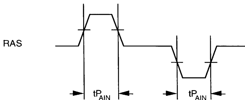
Fig. 36 Analog Receive Data Input Timing Diagram
