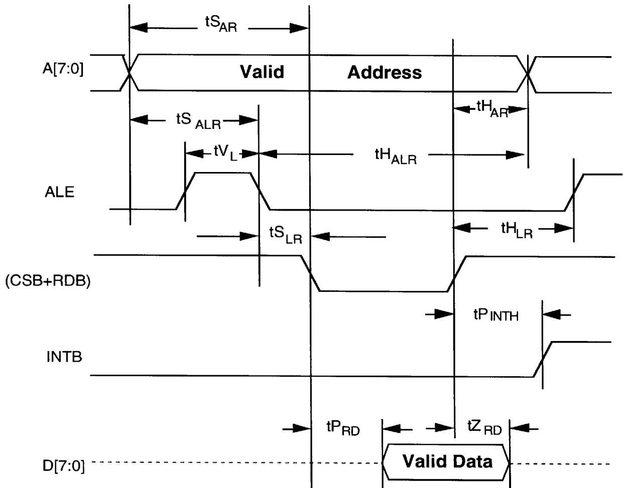
Fig. 22 Microprocessor Read Access Timing
