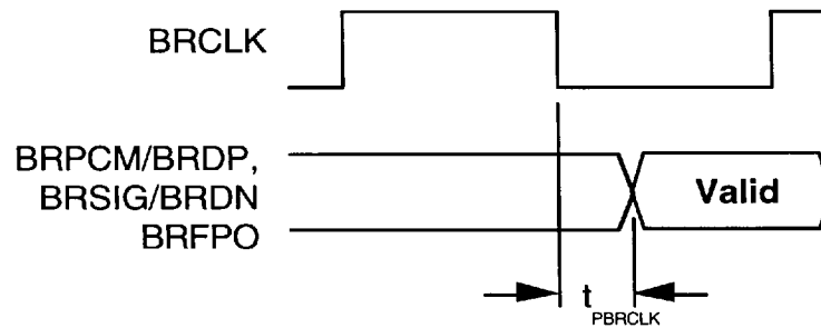
Fig. 31 Backplane Receive Output Timing Diagram
