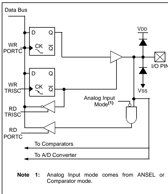
FIGURE 4-7: BLOCK DIAGRAM OF RC0 AND RC1
