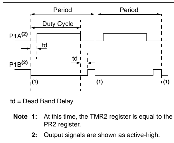
FIGURE 11-6: HALF-BRIDGE PWM OUTPUT
