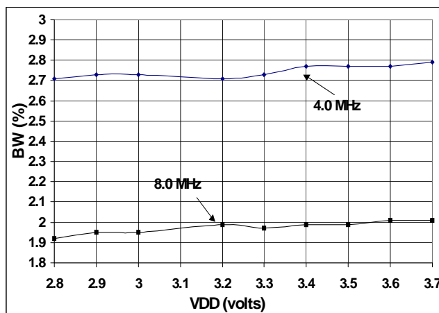
Bandwidth % vs. VDD
