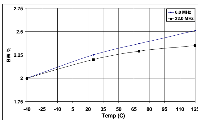
Bandwidth % vs. Temperature
