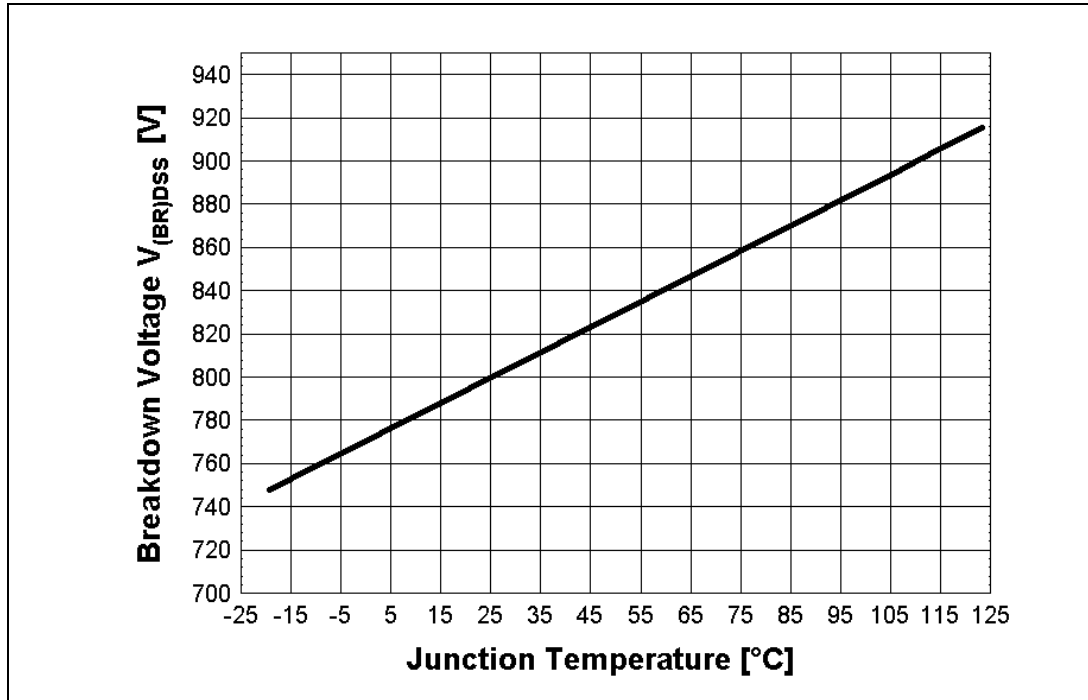
Figure 9 Drain-Source Breakdown voltage; V_{BR(DSS)} = f(T_j), I_D = 0.25mA
