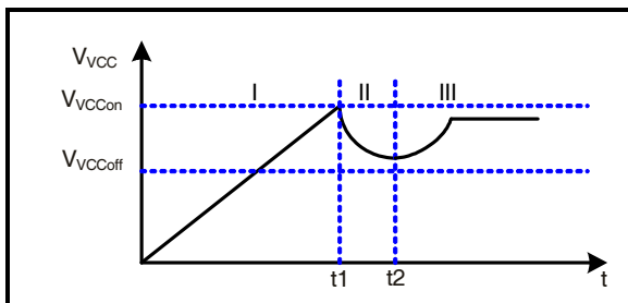
Figure 3 VCC voltage at start up
