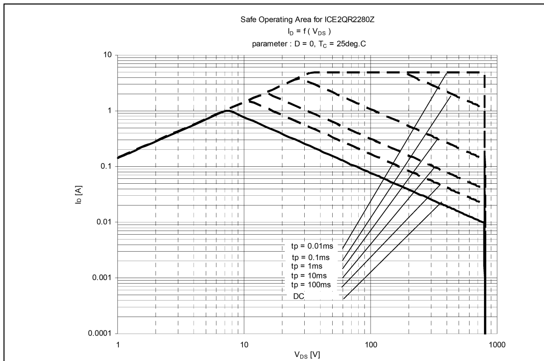
Figure 10 Safe Operating Area(SOA) for ICE2QR2280Z
