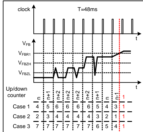
Figure 5 Up/down counter operation
