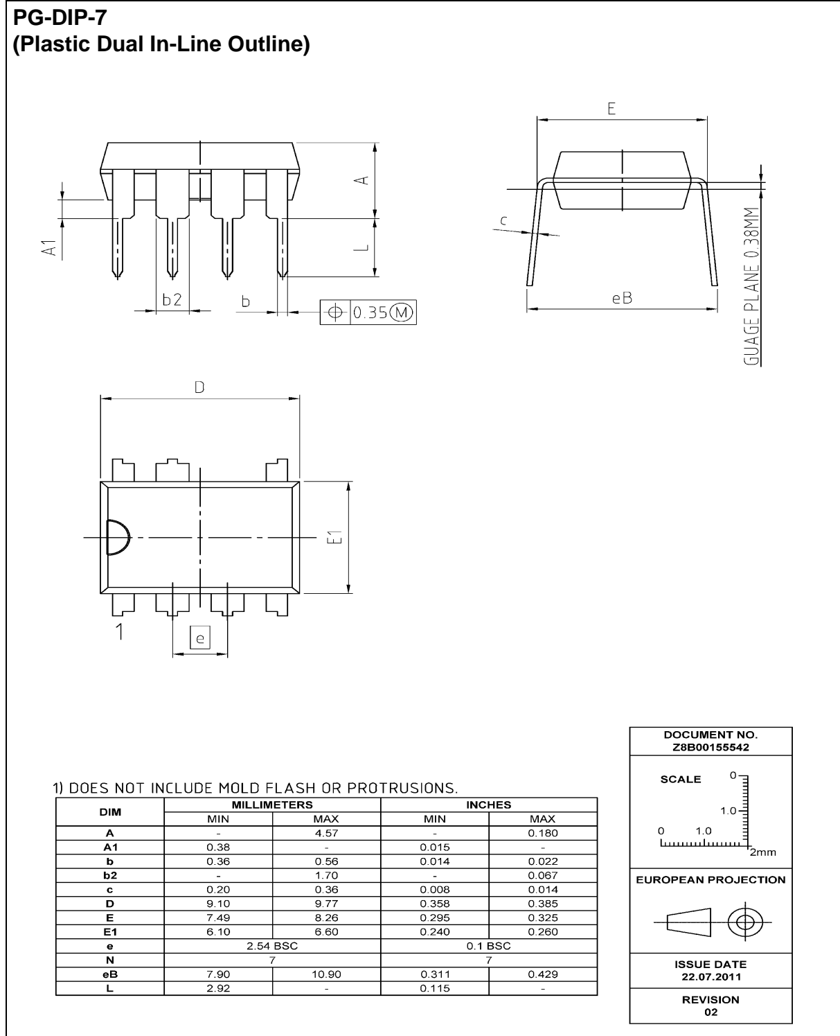
Figure 13 PG-DIP-7
