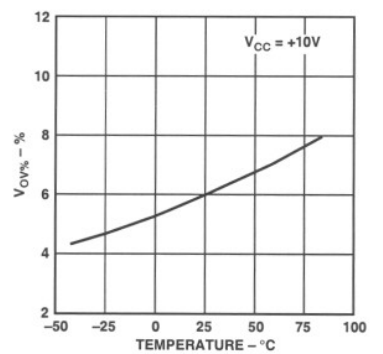
Figure 19. Overvoltage Comparator Threshold ( V_{OV\%} ) vs. Temperature
