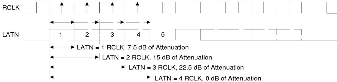
Figure 9. LATN Pulse Width encoding
