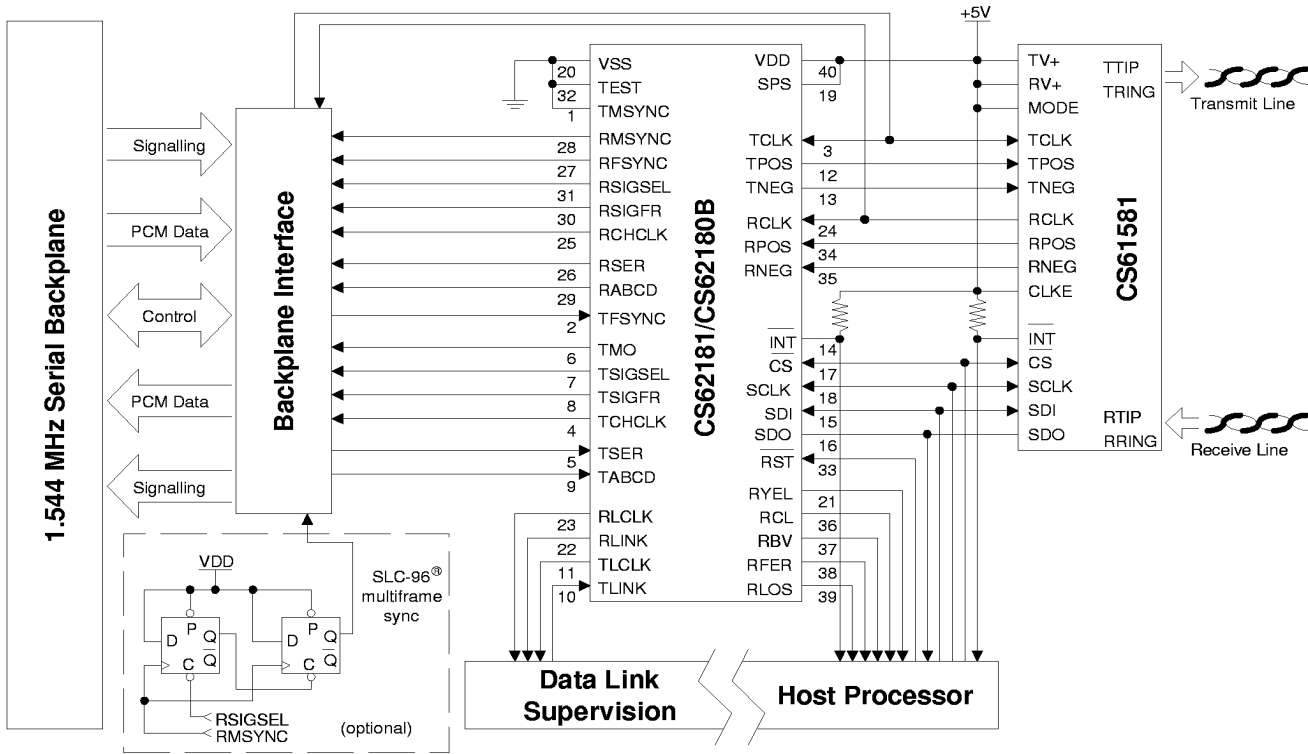
Figure 16. Typical System Connection
