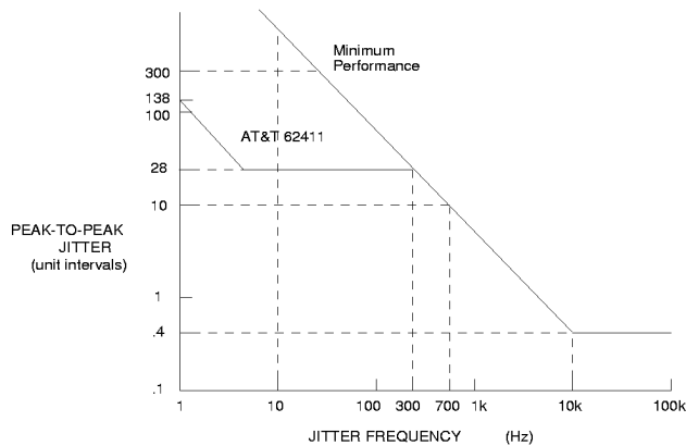
Figure 8. Minimum Input Jitter Tolerance of Receiver
