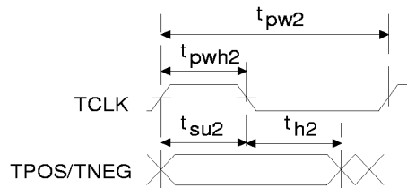
Figure 3. Transmit Clock and Data Switching Characteristics
