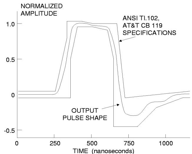
Figure 6. Typical Pulse Shape at DSX-1 Cross Connect
