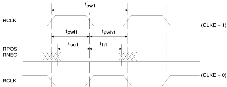
Figure 2. Recovered Clock and Data Switching Characteristics
