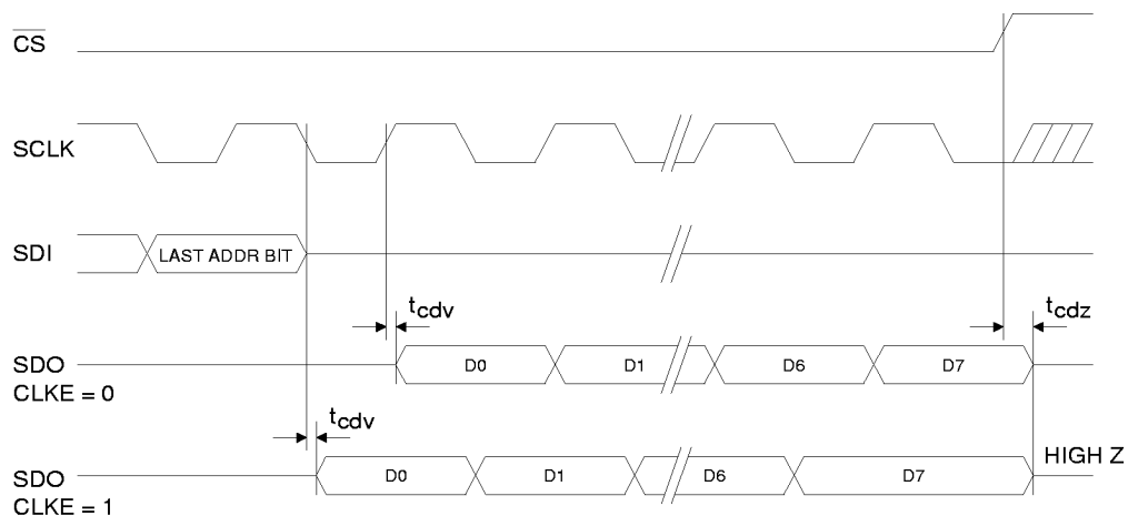
Figure 5. Serial Port Read Timing Diagram
