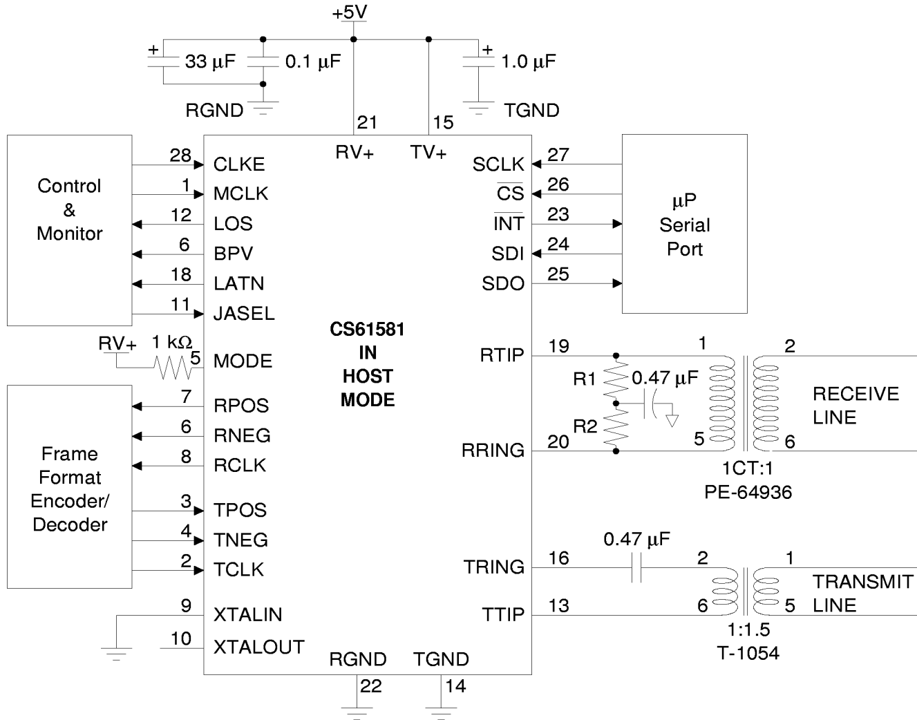
Figure 14. Matched Impedance Output Configuration
