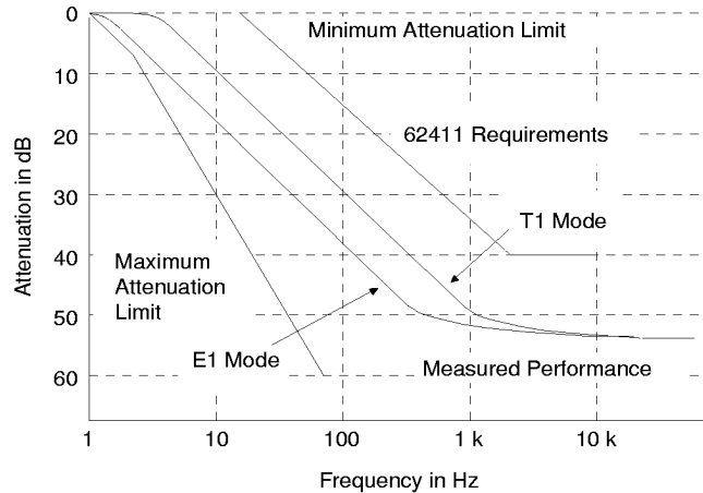
Figure 10. Typical Jitter Transfer Function
