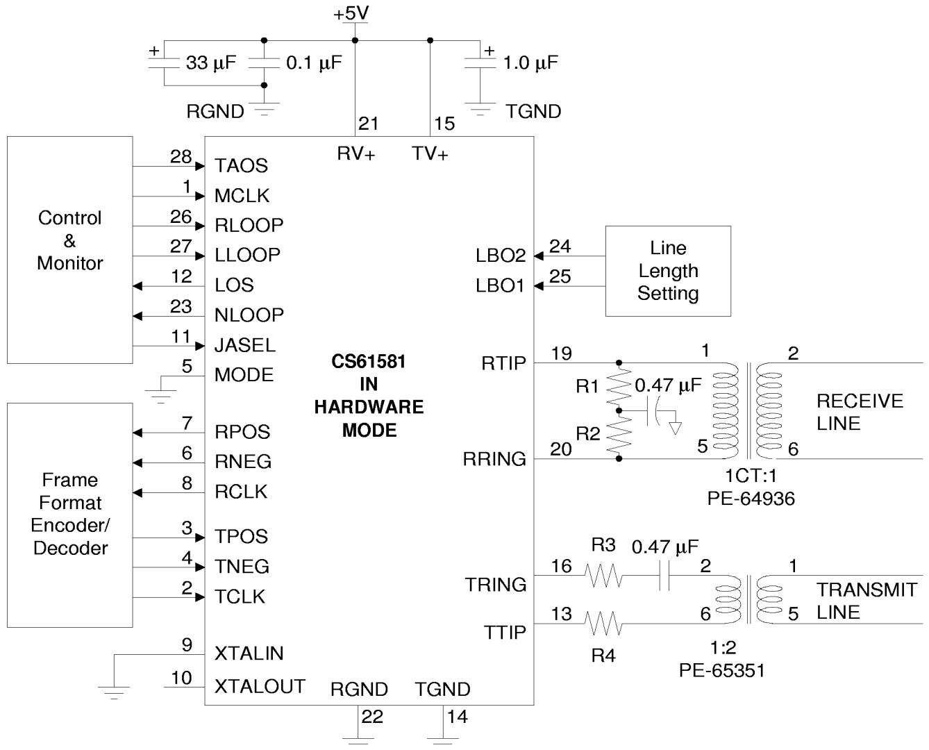
Figure 15. Low Impedance Output Configuration
