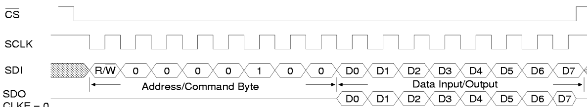
Figure 11. Input/Output Timing (showing address 0x10)
