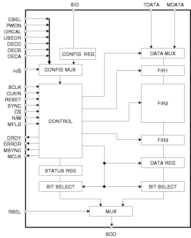
Figure 19. CS5322 Block Diagram
