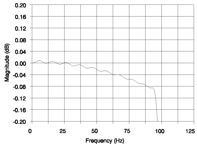
Figure 6. CS5322 Digital Filter Passband Ripple f_0 = 250\text{ Hz}
