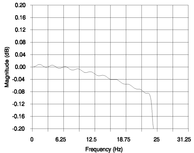
Figure 4. CS5322 Digital Filter Passband Ripple f_0 = 62.5\text{ Hz}
