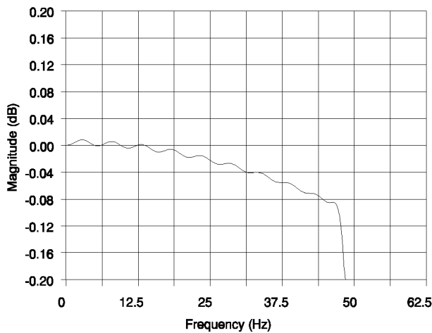
Figure 5. CS5322 Digital Filter Passband Ripple f_0 = 125\text{ Hz}
