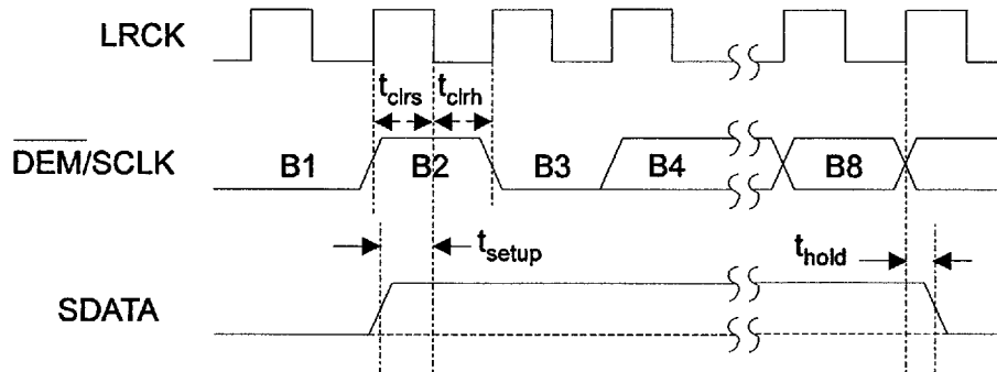
Figure 22. Configuration Timing
