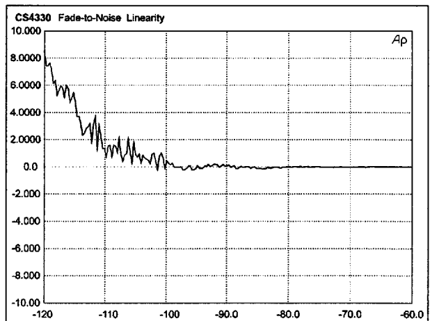
Figure 20. Fade-to-Noise Linearity
