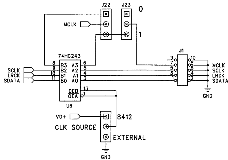
Figure 5. I/O Interface for Clocks and Data
