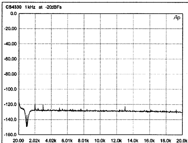
Figure 17. -20 dBfs FFT
