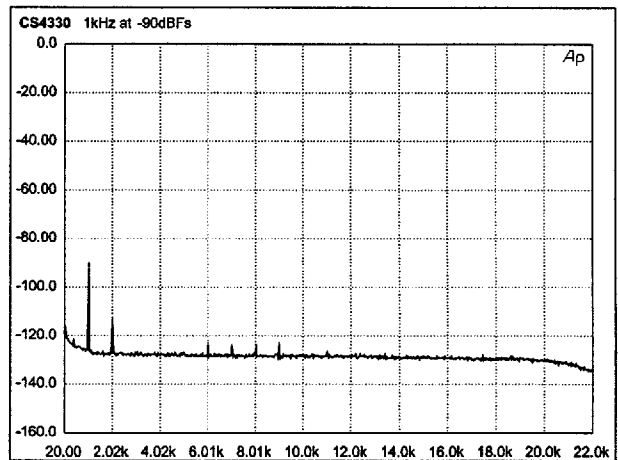
Figure 19. -90 dBfs FFT
