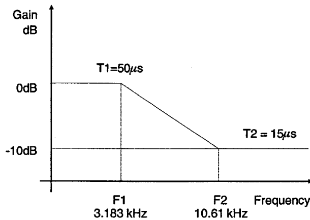
Figure 3. De-Emphasis Curve ( F_s = 44.1\text{kHz} )
