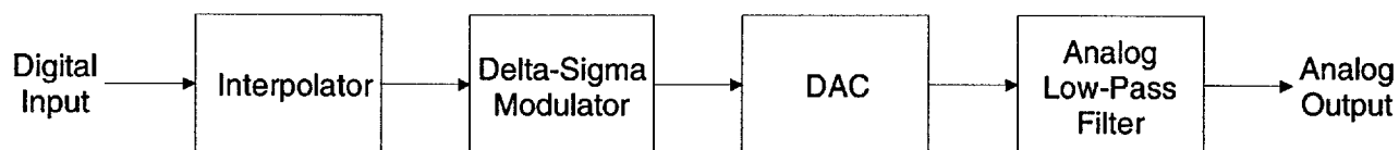
Figure 2. System Block Diagram
