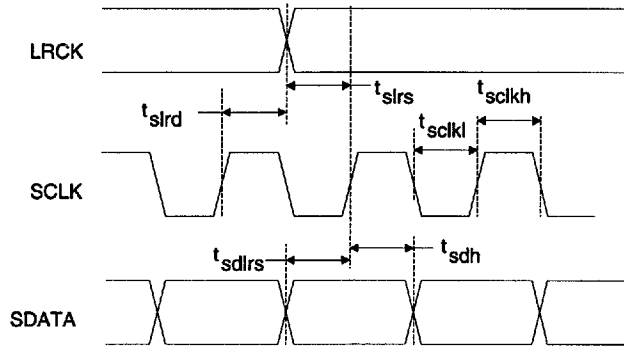
External Serial Mode Input Timing
