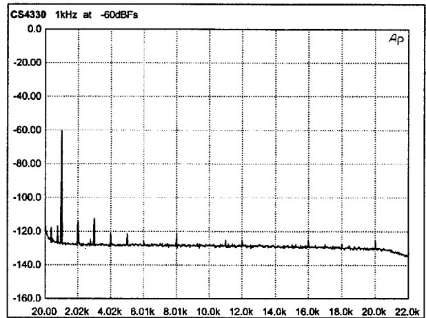
Figure 18. -60 dBfs FFT
