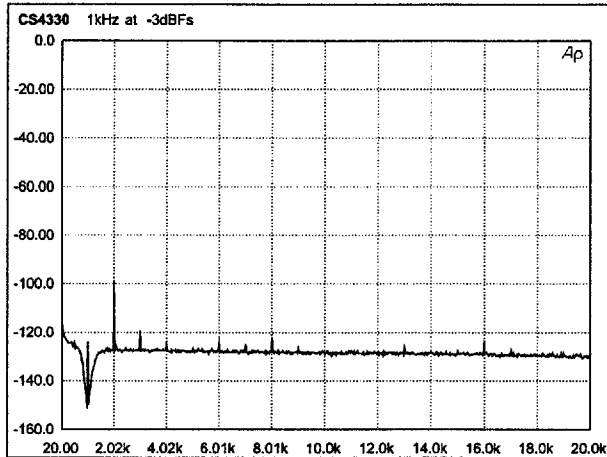
Figure 16. -3 dBfs FFT
