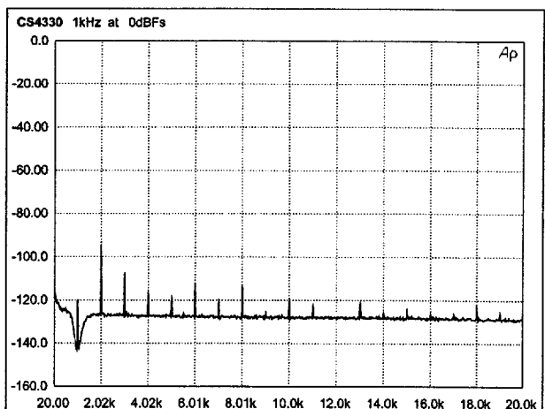
Figure 15. 0 dBFS FFT
