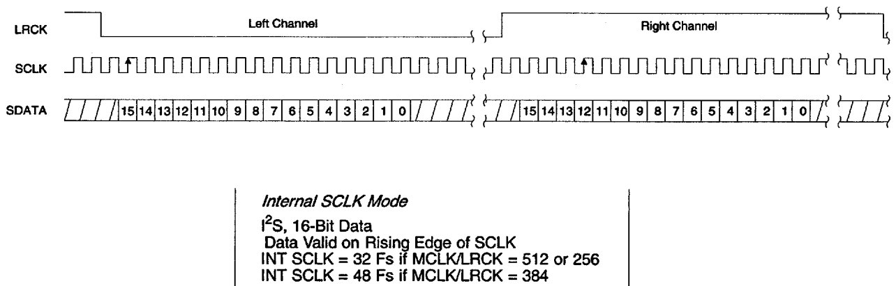
Figure 5. CS4331 Internal SCLK Data Format (I 2 S)
