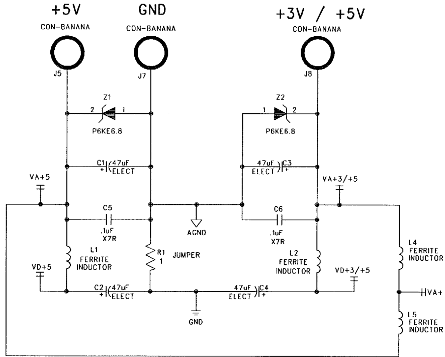
Figure 7. Power Supply
