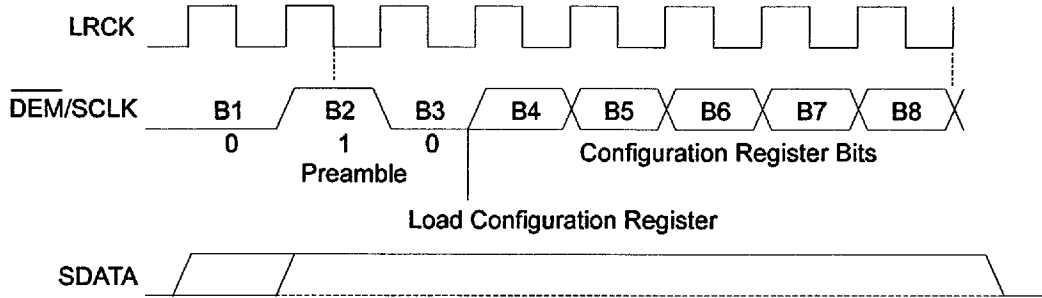
Figure 21. Configuration Operation
