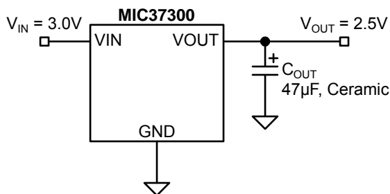
Fixed 2.5V Regulator
