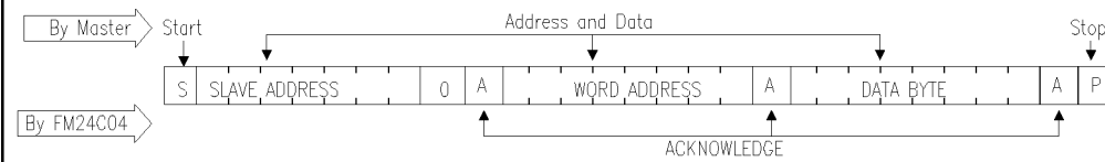
Figure 5 Byte Write
