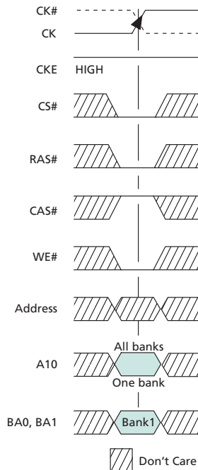
Figure 18: PRECHARGE Command
