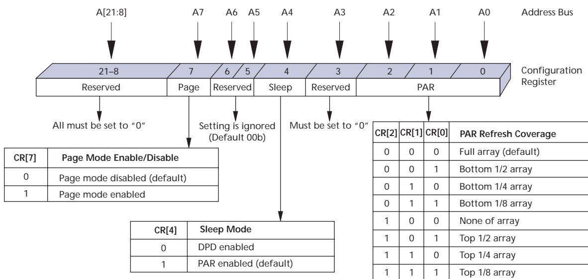
Figure 9: Configuration Register Definition
