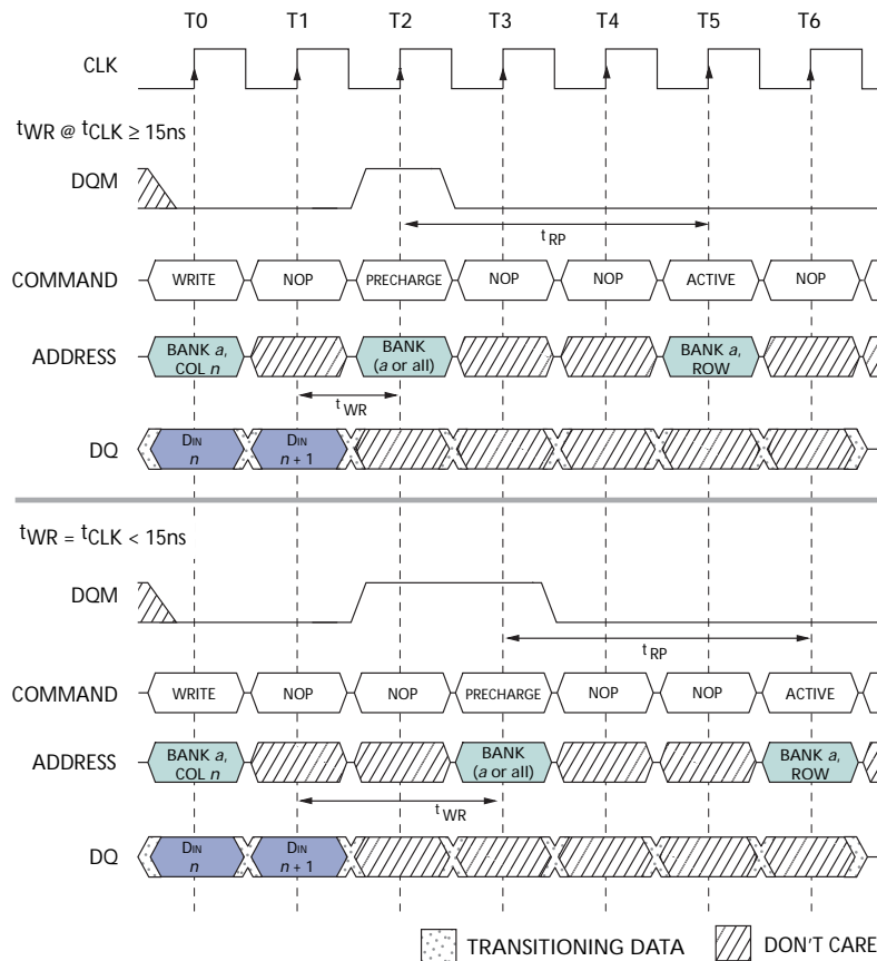
Figure 25: WRITE-To-PRECHARGE
