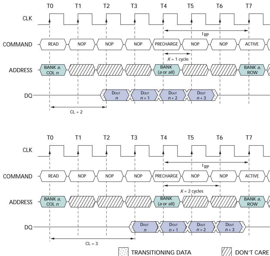
Figure 18: READ-to-PRECHARGE
