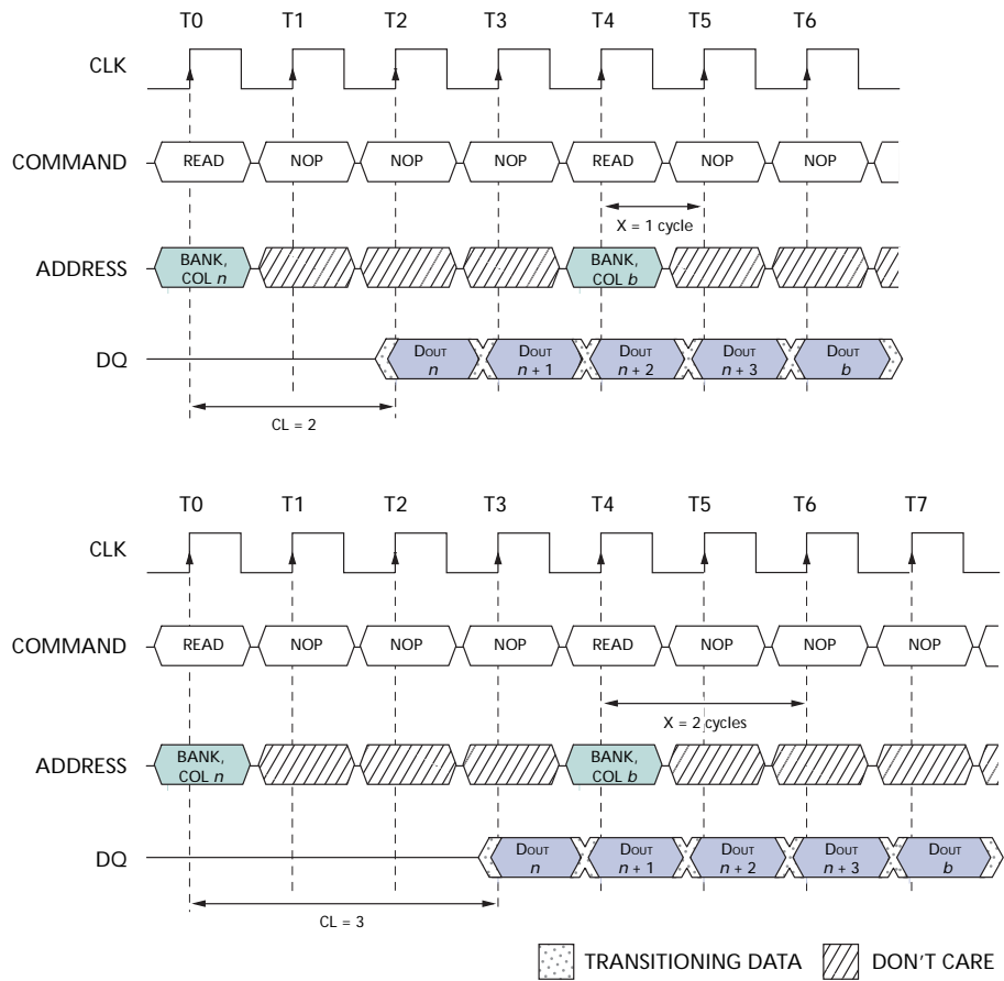
Figure 14: Consecutive READ Bursts
