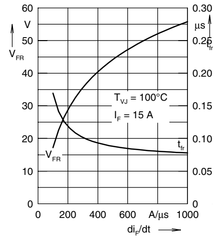
Fig. 6 Peak forward voltage V_{FR} / t_{tr} versus di_F/dt
