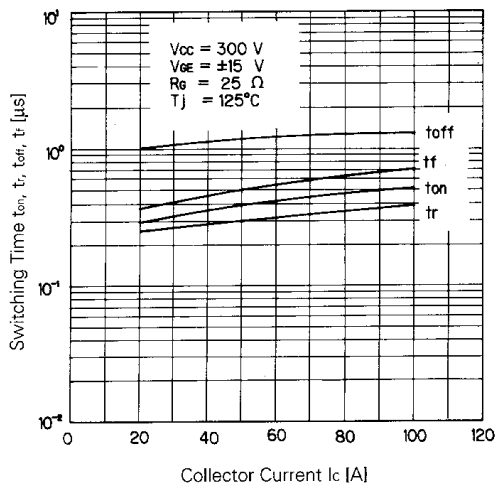
Switching Time
