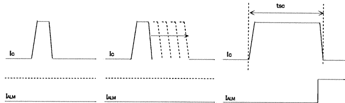
Fig3 Definition of tsc
