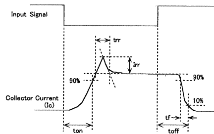
Fig4 Definition of Switching Time
