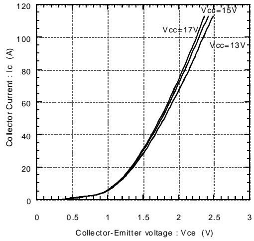
Collector current vs. Collector-Emitter voltage Tj=25°C(Terminal)
