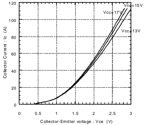
Collector current vs. Collector-Emitter voltage Tj=125°C(Terminal)
