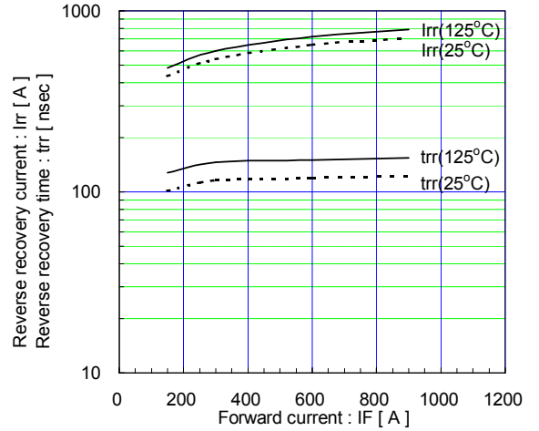
Reverse recovery characteristics (typ.) Vcc=600V, VGE=±15V, RG=0.6Ω
