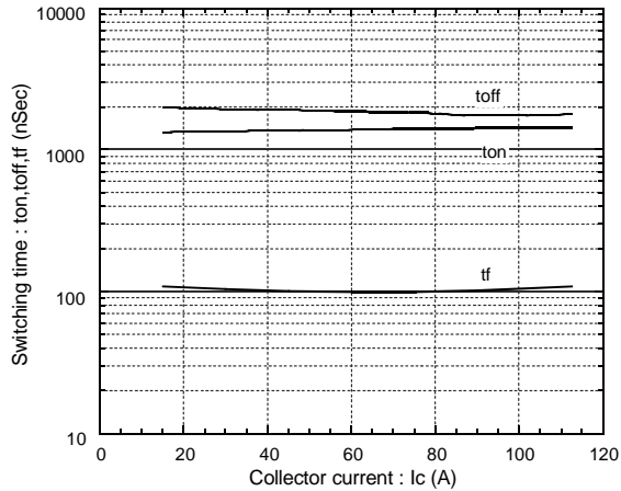
Switching time vs. Collector current E dc =600V, V cc =15V, T j =25°C
