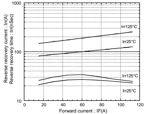
Reverse recovery characteristics trr, Irr vs. IF
