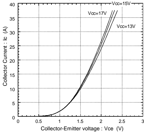
Collector current vs. Collector-Emitter voltage Tj=25°C
