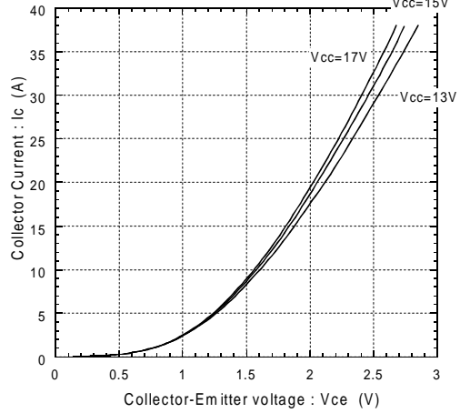
Collector current vs. Collector-Emitter voltage Tj=125°C
