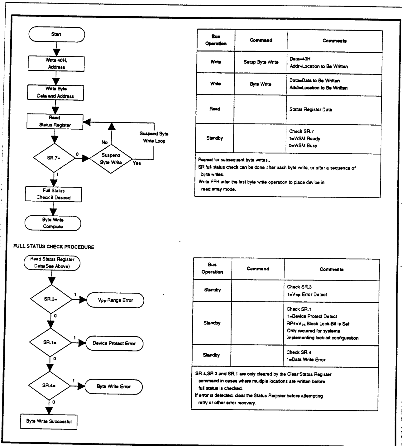
Figure 6. Automated Byte Write Flowchart
