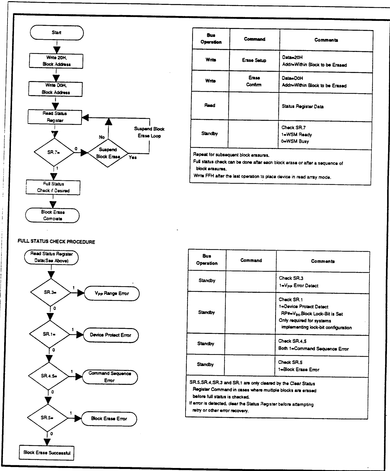
Figure 5. Automated Block Erase Flowchart
