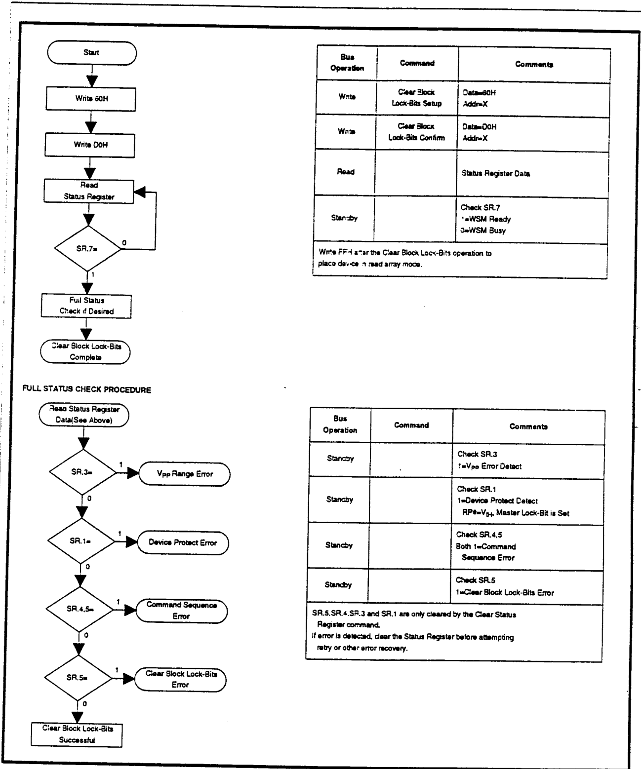
Figure 10. Clear Block Lock-Bits Flowchart
