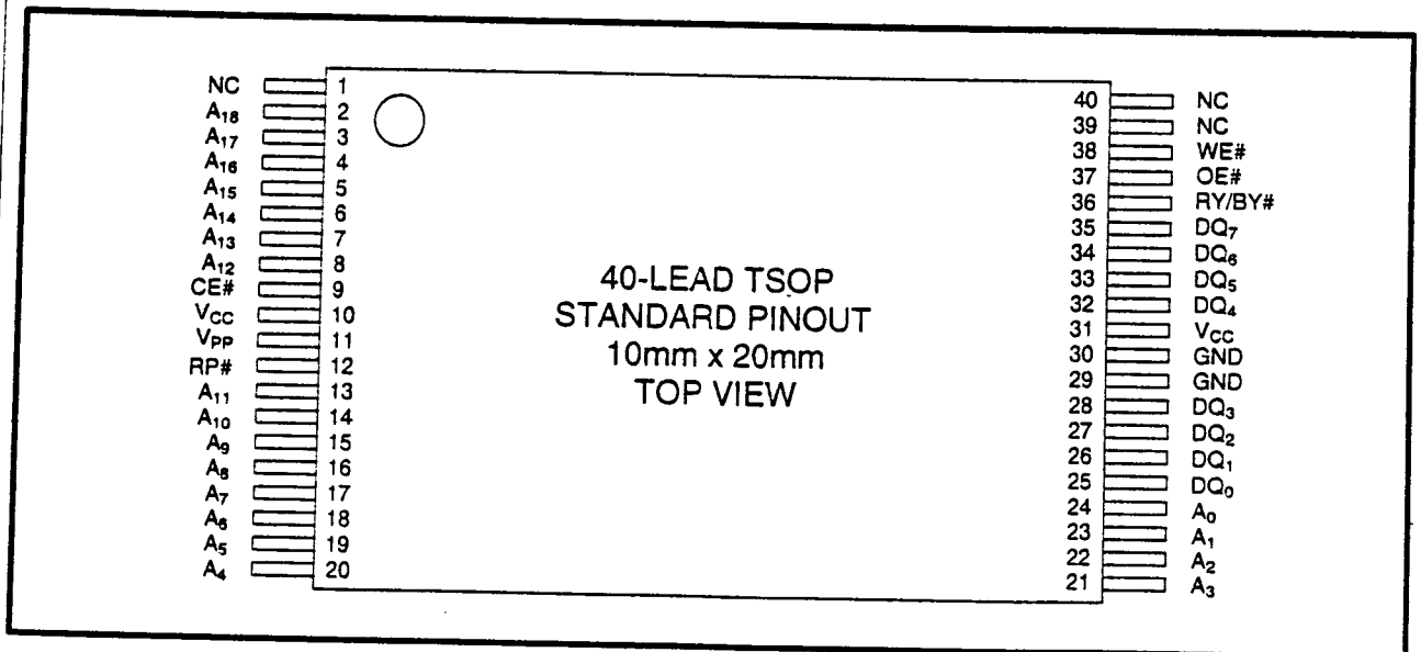
Figure 2. TSOP 40-Lead Pinout
