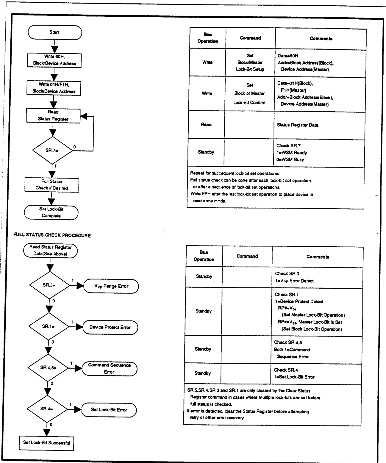
Figure 9. Set Block and Master Lock-Bit Flowchart
