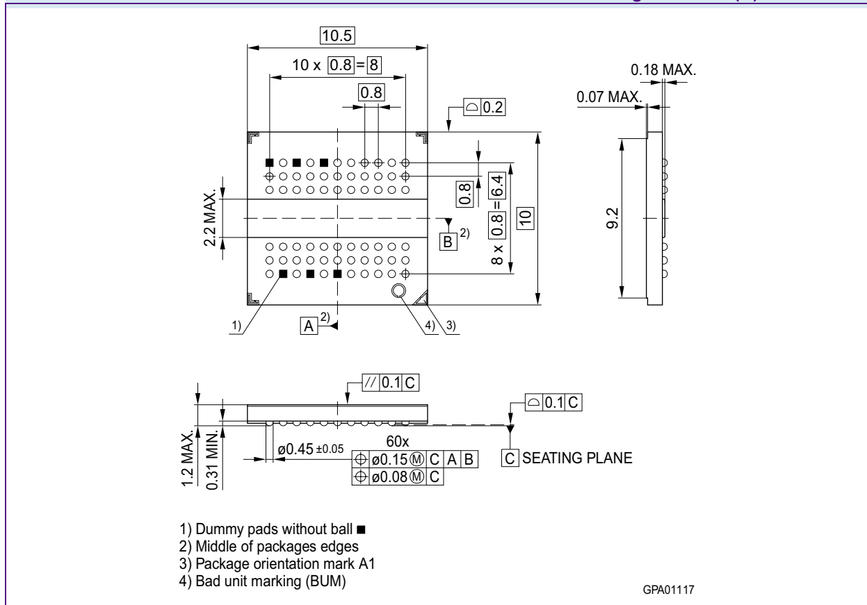
FIGURE 13 Package Outline P(G)-TFBGA-60-6
