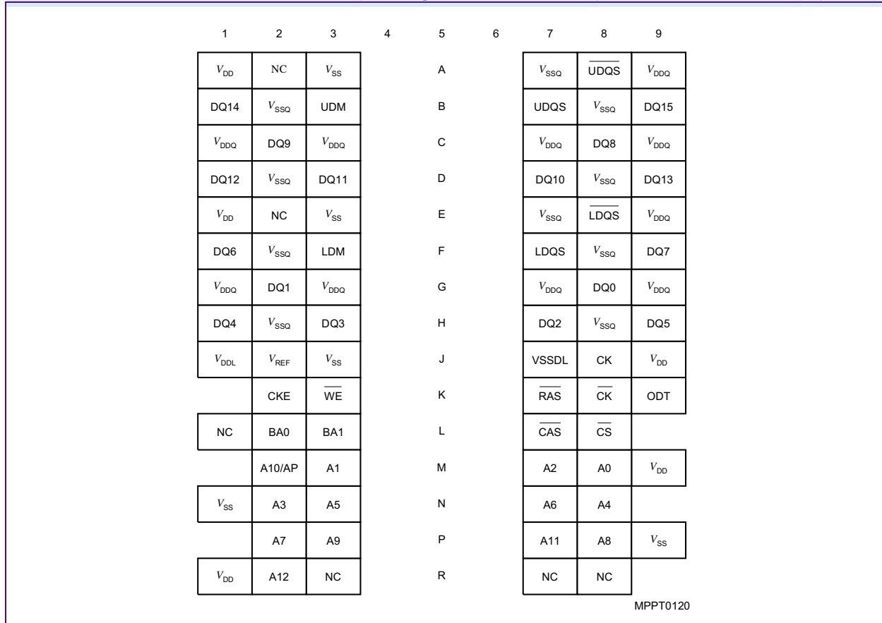
Chip Configuration for ×16 components, PG-TFBGA-84 (top view)
