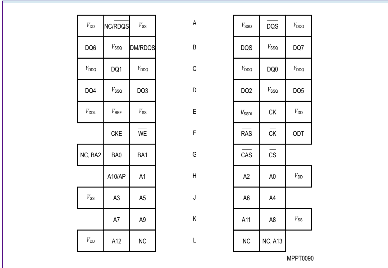
Chip Configuration for ×8 components, PG-TFBGA-60 (top view)
