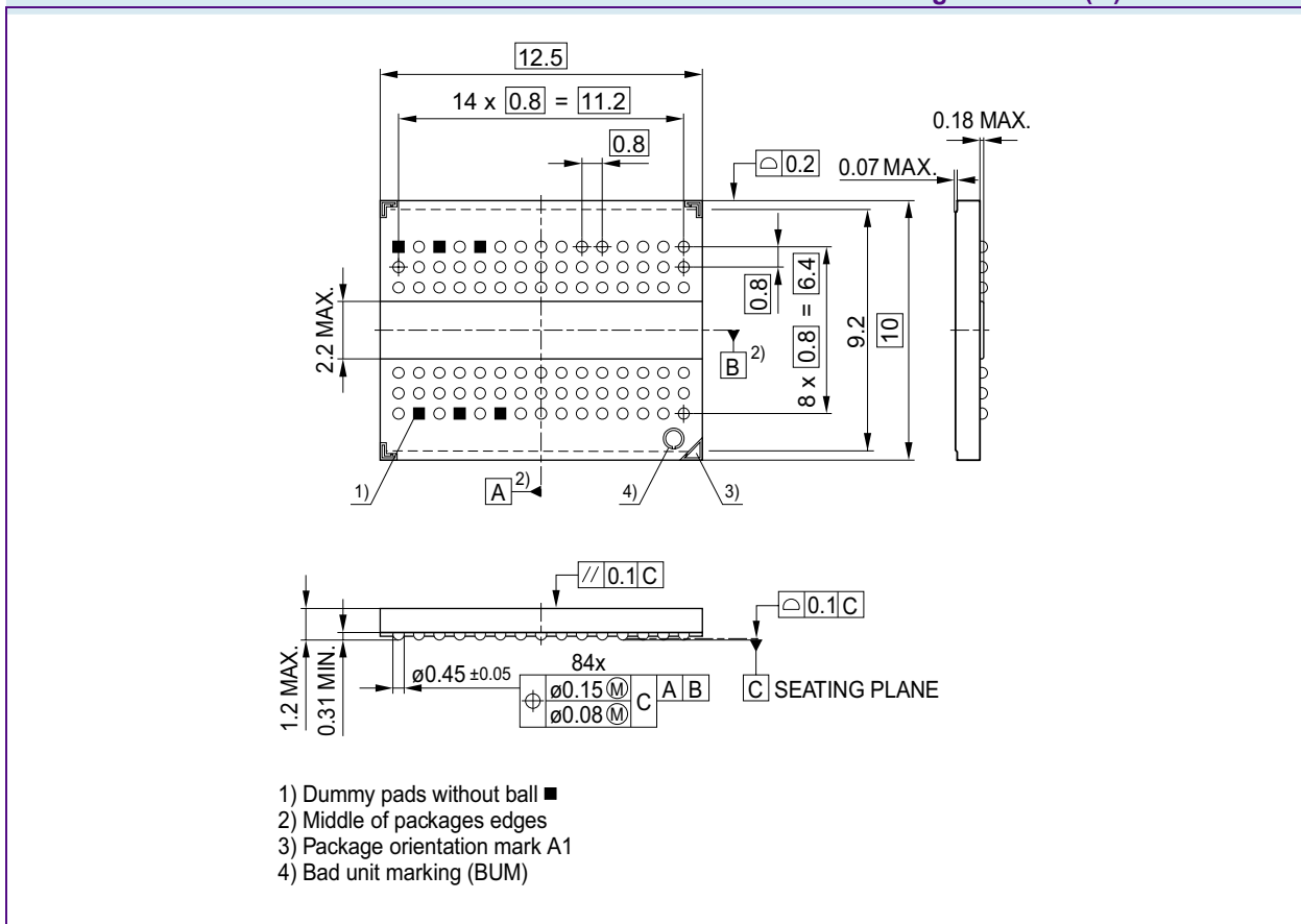
FIGURE 11 Package Outline P(G)-TFBGA-84-51
