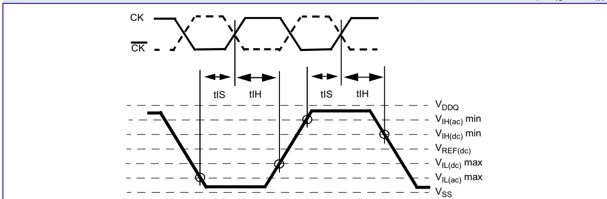
Differential input waveform timing - t_{IS} and t_{IH}
