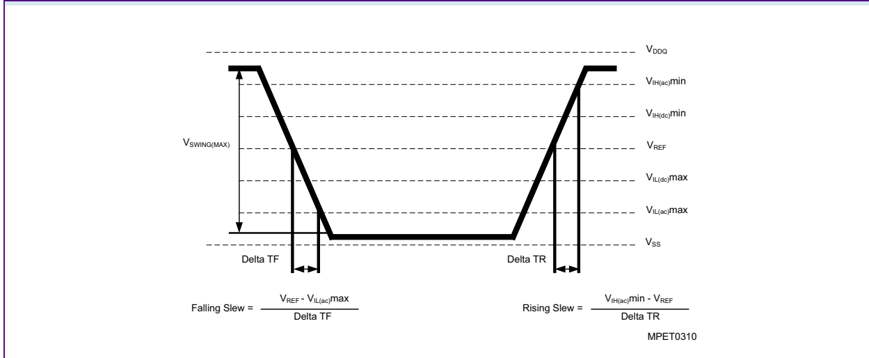
Single-ended AC Input Test Conditions Diagram
