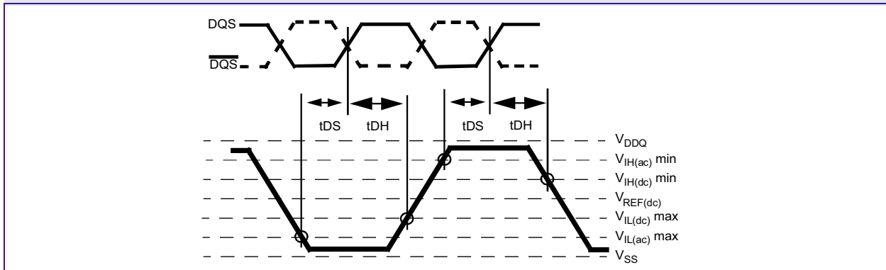
Differential input waveform timing - t_{DS} and t_{DH}
