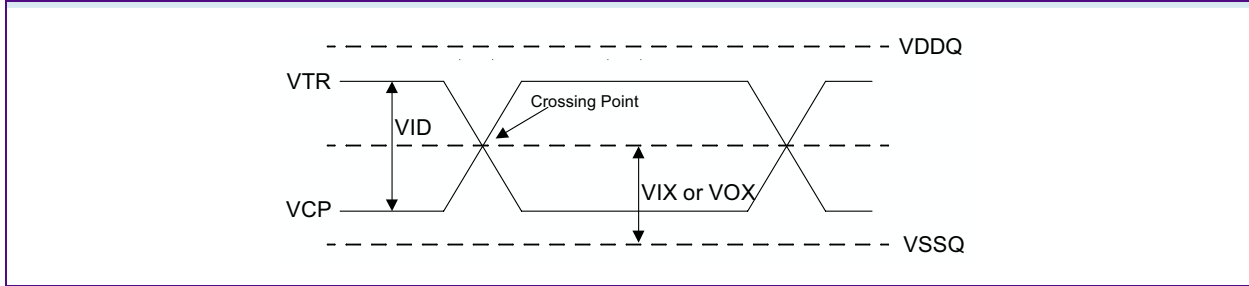
Differential DC and AC Input and Output Logic Levels Diagram
