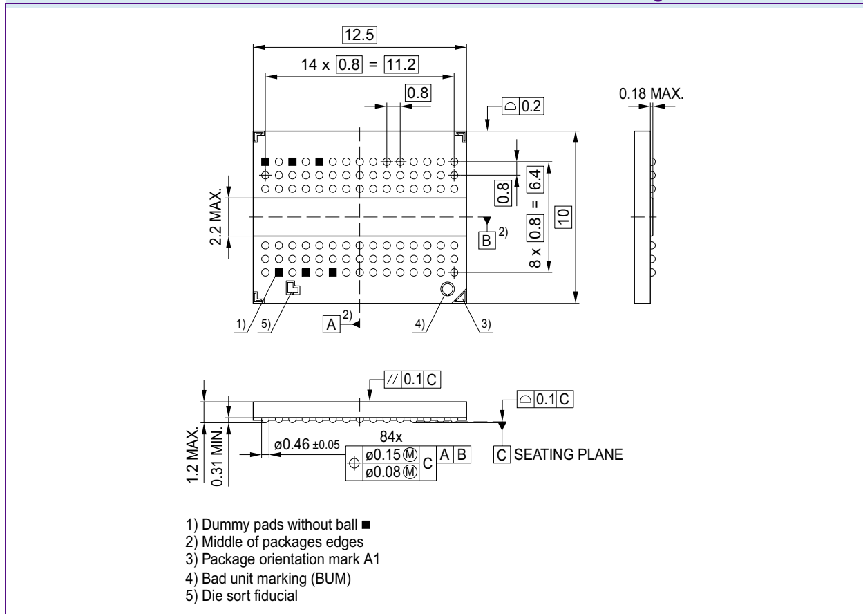
FIGURE 12 Package Outline P-TFBGA-84-1
