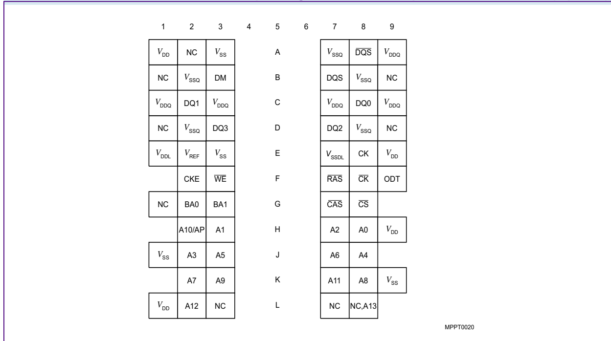
Chip Configuration for ×4 components, PG-TFBGA-60 (top view)
