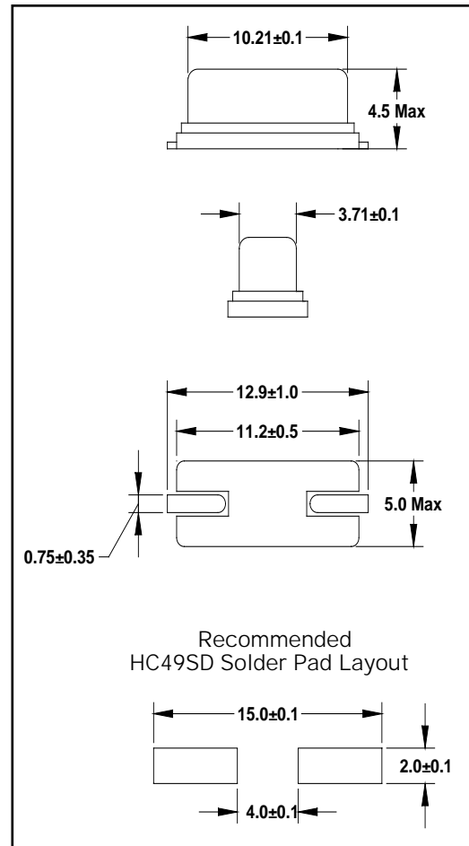
All dimensions are in millimeters. TERMINATION FINISH: Sn/3.0Ag/0.5Cu
