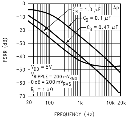
Power Supply Rejection Ratio Mic Preamp
