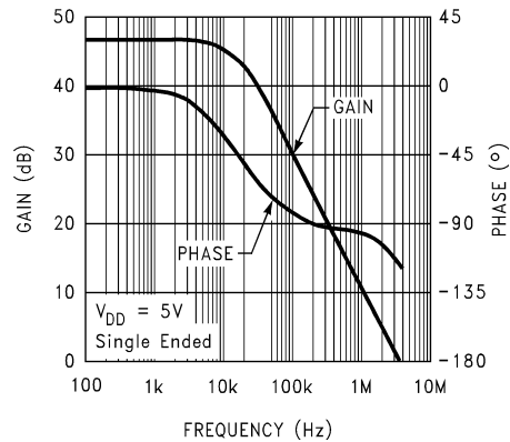
Open Loop Frequency Response Bridged Power Amp
