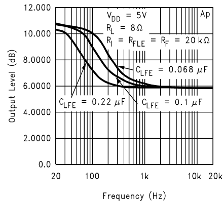
Low Frequency Enhancement Characteristics Bridged Power Amp
