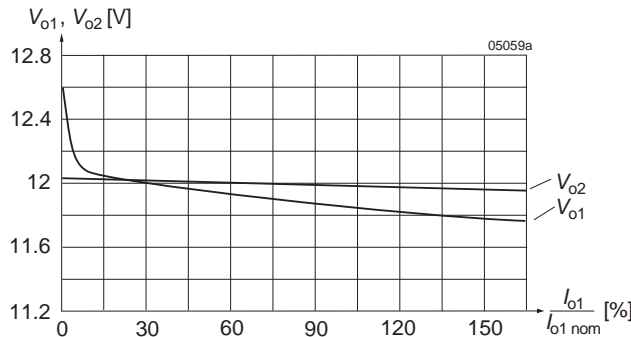
Fig. 10 Flexible load distribution on double-outputs models (2 × 12 V) with load variation from 0 to 150% of P_{o1\ nom} on output 1. Output 2 loaded with 25% of P_{o2\ nom} .
