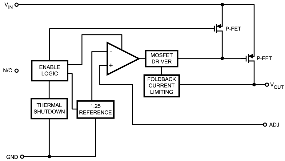
FIGURE 1. LP38691-ADJ Functional Diagram (LLP)
