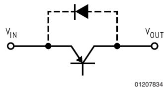
FIGURE 4. LP2980 Reverse Current Path
