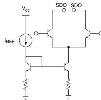
Fig. 2 Differential Output Stage, I_{\text{REF}} Derived using R_{\text{SET}}
