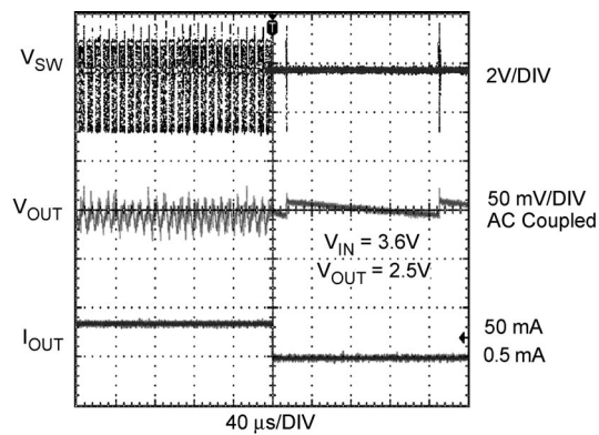
Load Transient Response ( V_{OUT} = 2.5V ) (PFM Mode 50mA to 0.5mA)
