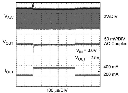
Load Transient Response V_{OUT} = 2.5V (PWM Mode)
