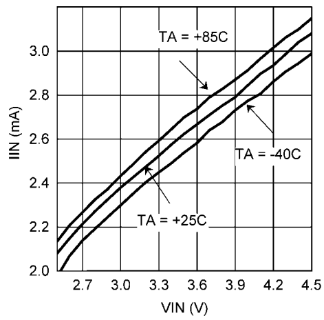
Active (Switching) Supply Current vs V_{IN} ( V_{OUT} = 5V, I_{OUT} = 400mA )
