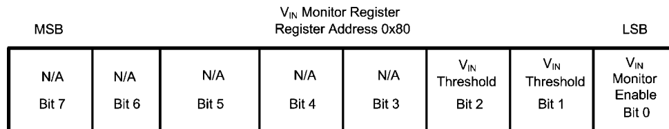
FIGURE 23. V IN Monitor Register Description
