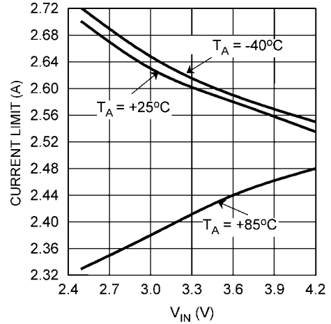
Closed Loop Current Limit vs V_{IN} (Flash Duration Register bits [6:5] = 11, (Note 8))
