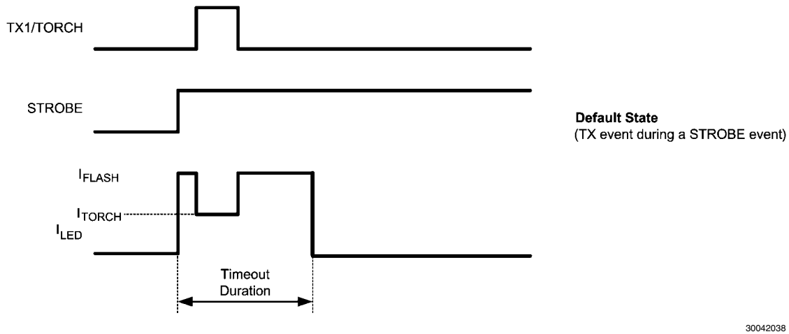
FIGURE 4. TX1 Event During a Flash Event (Default State, TX1/TORCH is an Active High TX Input)
