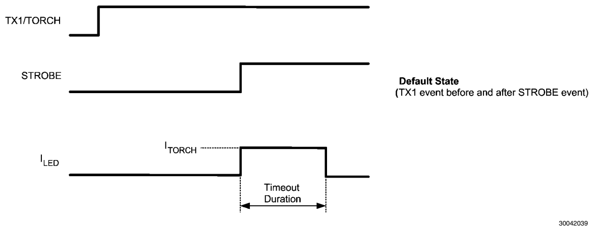
FIGURE 5. TX1 Event Before and After Flash Event (Default State, TX1/TORCH is an Active High TX Input)
