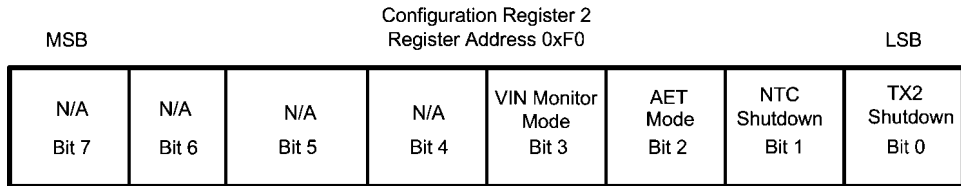
FIGURE 21. Configuration Register 2 Description
