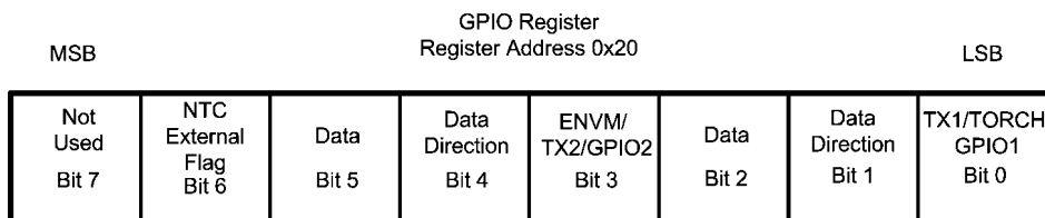
FIGURE 22. GPIO Register Description
