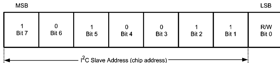
FIGURE 15. Device Address
