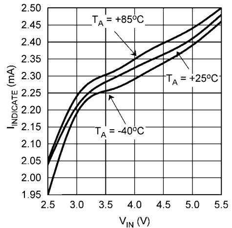
Indicator Current vs V_{IN} , V_{LEDI} = 2V (Torch Brightness Register bits [7:6] = 00)
