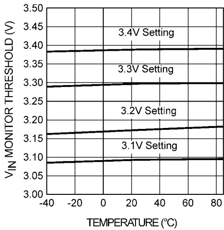
V_{IN} Monitor Thresholds vs Temperature
