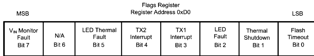
FIGURE 19. Flags Register Description
