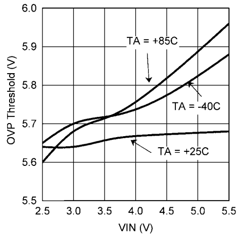
OVP Thresholds vs V_{IN} (Note 9)
