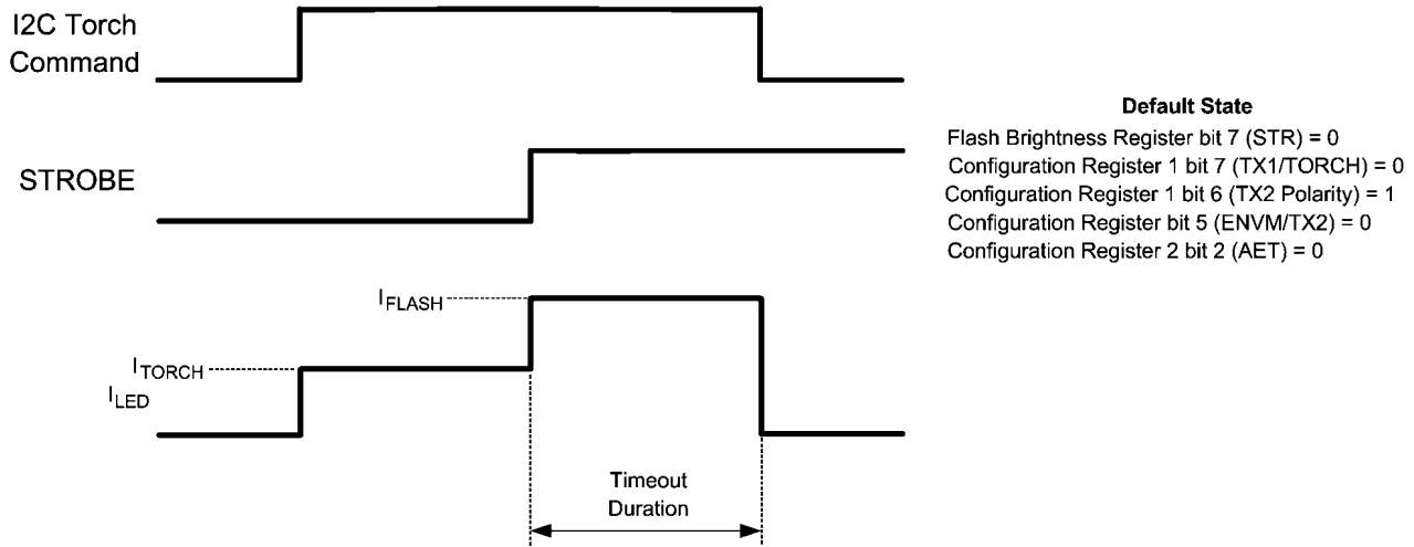
FIGURE 3. Normal Torch to Flash Operation (Default, Power On or RESET state of LM3554)
