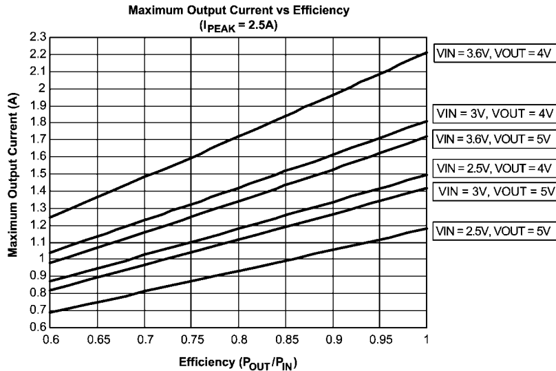
FIGURE 2. LM3554 Maximum Output Current
