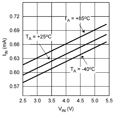
Active (Non-Switching) Supply Current vs V_{IN} ( V_{LED} = 1.5V )
