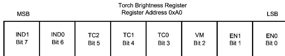
FIGURE 16. Torch Brightness Register Description
