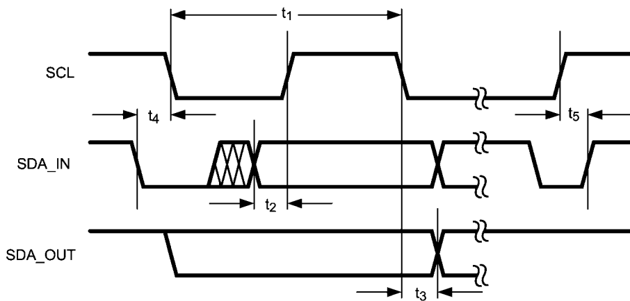
FIGURE 1. I 2 C Timing
