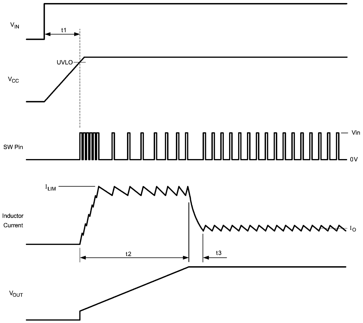
FIGURE 2. Startup Sequence
