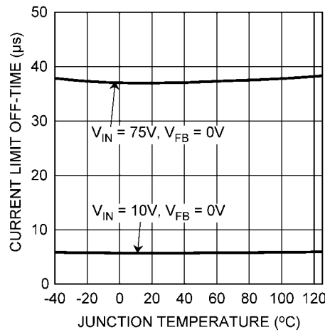
Current Limit Off-Time vs. Temperature
