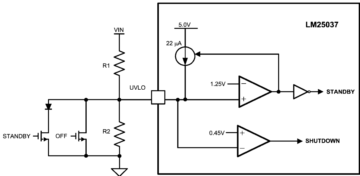
FIGURE 15. Remote Standby and Disable Control
