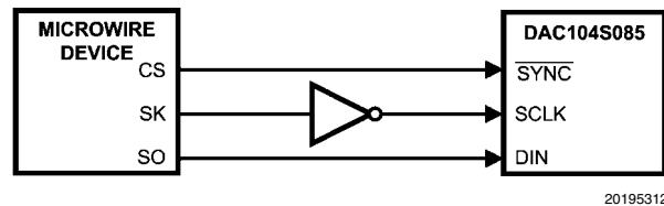
FIGURE 13. Microwire Interface
