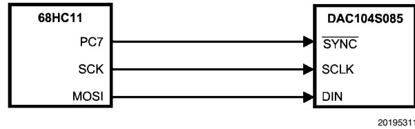
FIGURE 12. 68HC11 Interface
