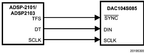
FIGURE 10. ADSP-2101/2103 Interface
