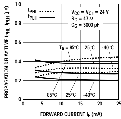
Figure 42. Typical propagation delay time vs. forward current, HCPL-3100.
