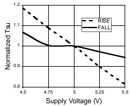
Normalized Tsu vs Vcc
