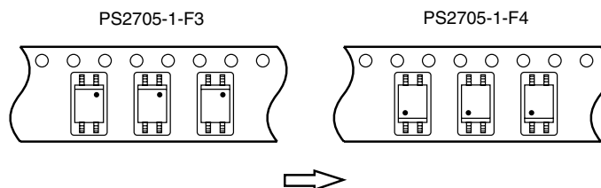
Tape Direction
