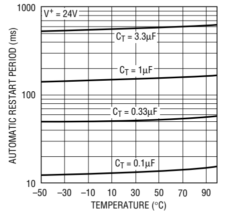
Automatic Restart Period vs Temperature
