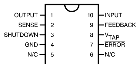
10-Lead Ceramic Surface-Mount Package (WG)
