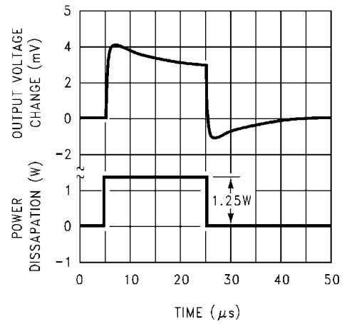
Thermal Response
