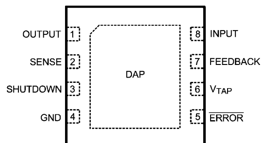
8-Lead LLP
