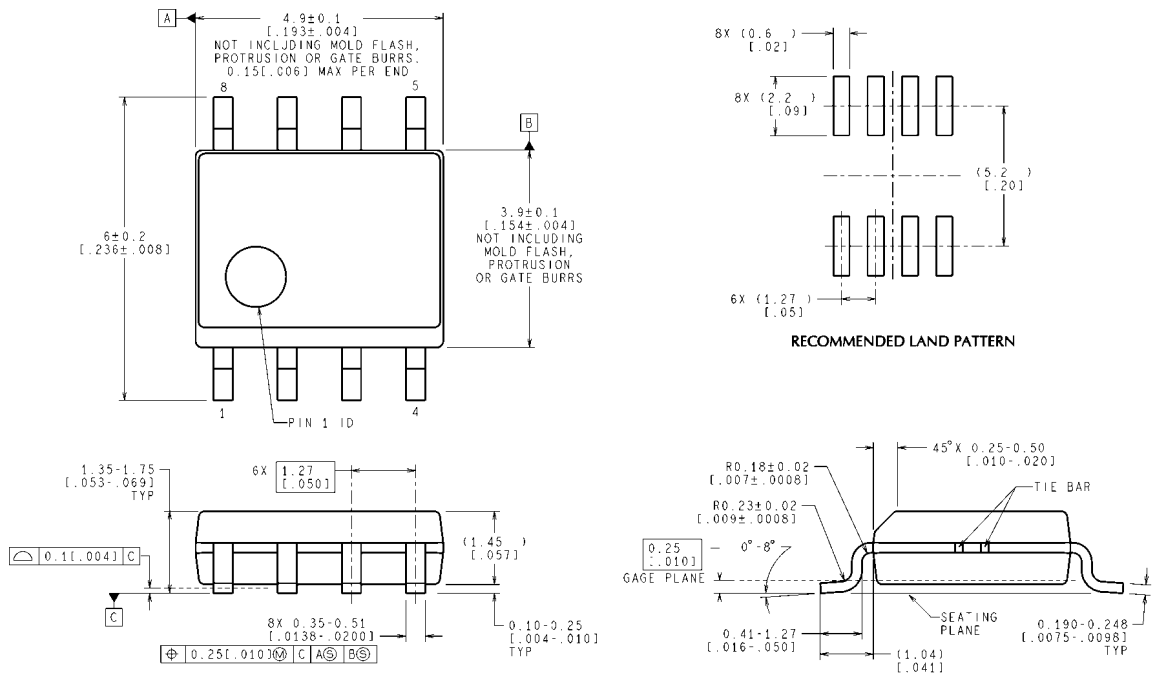
Surface Mount Package (M) NS Package Number M08A
