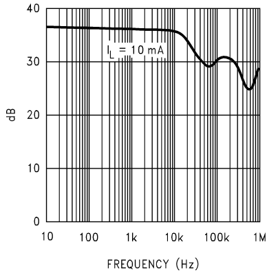
Ripple Rejection
