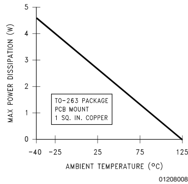
FIGURE 4. Maximum Power Dissipation vs. T_{\text{AMB}} for the TO-263 Package
