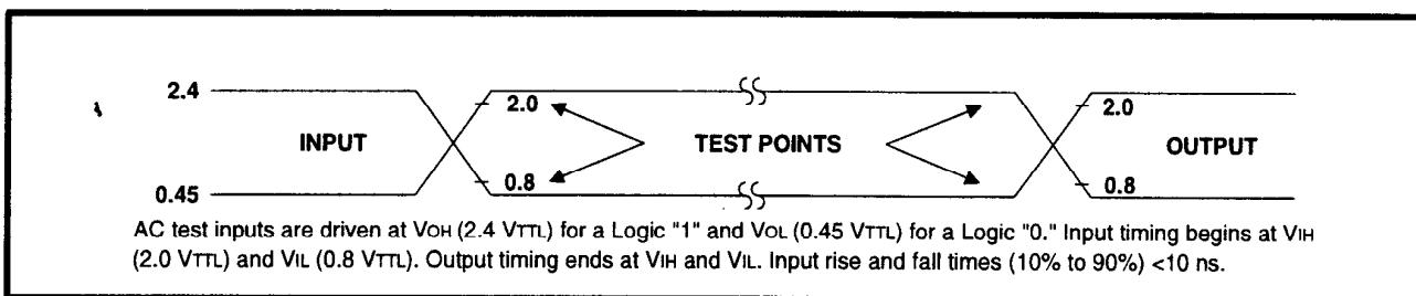
Figure 15. Transient Input/Output Reference Waveform for V_{CC}=5V\pm0.5V (Standard Testing Configuration)
