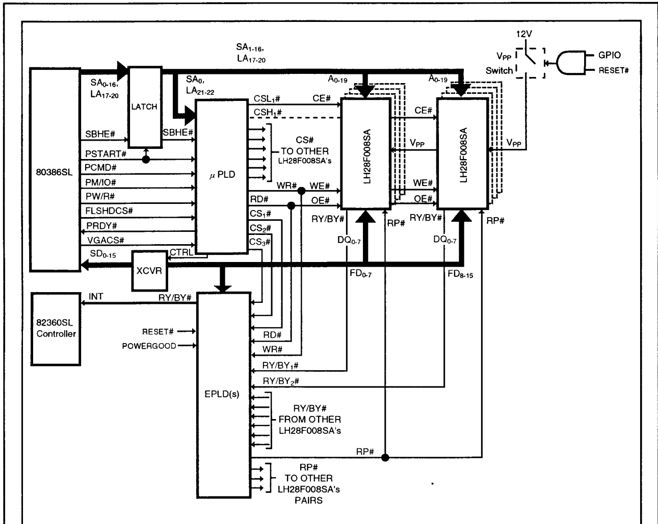
Figure 3. LH28F008SA Array Interface to 386SL Microprocessor Superset through PI Bus (Including RY/BY# Masking and Selective Powerdown), for DRAM Backup during System SUSPEND, Resident O/S and Applications and Motherboard Solid-State Disk.
