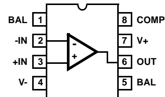
HA-2520, HA-2525 (8 LD CERDIP, 8 LD PDIP, CERDIP, SOIC) TOP VIEW
